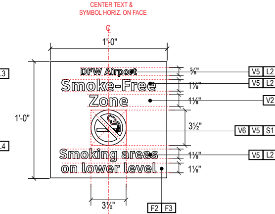
B DETAIL B: No Smoking Face Layout NTS
