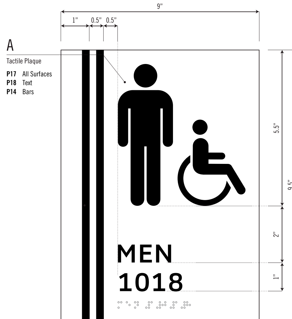
3 Elevation / Half Size Style A
