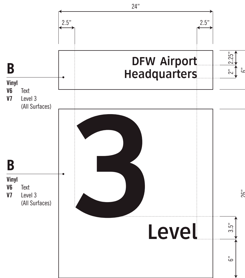
2 Elevation / 1 1/2" = 1'-0" Level 3
