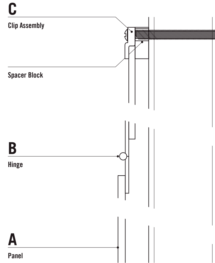
B Section Detail / NTS Clip Assembly
