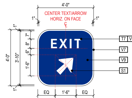
A10 FACE LAYOUT - *Typical Example (S-NB-7 shown) Scale: 1/4" = 1'-0"
