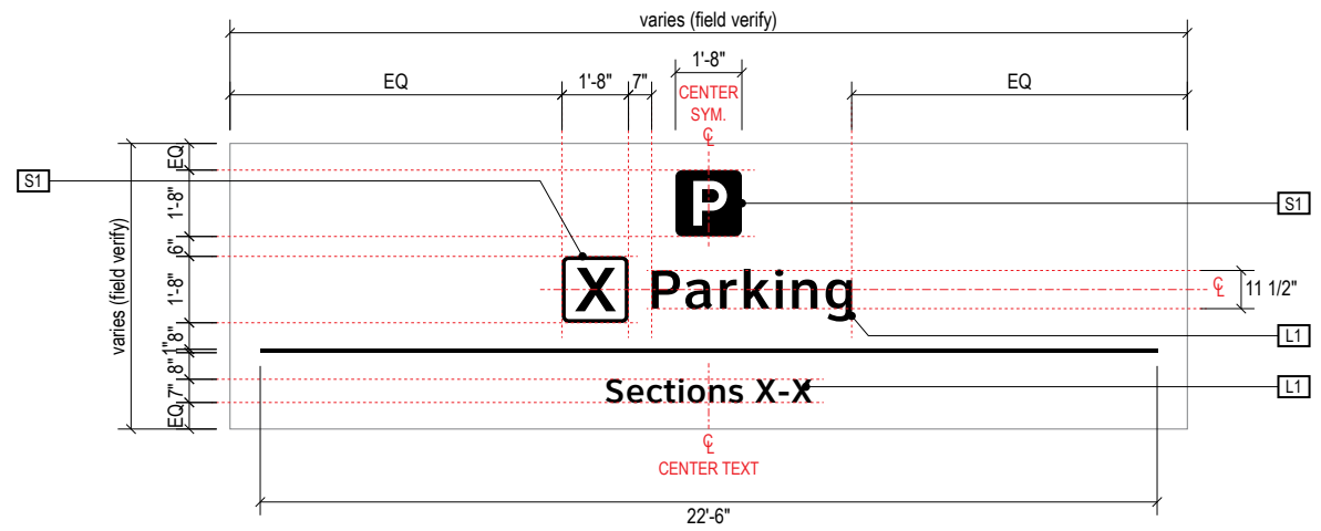
A DETAIL A: Face Layout (Typical) Scale: 3/16" = 1'-0"
