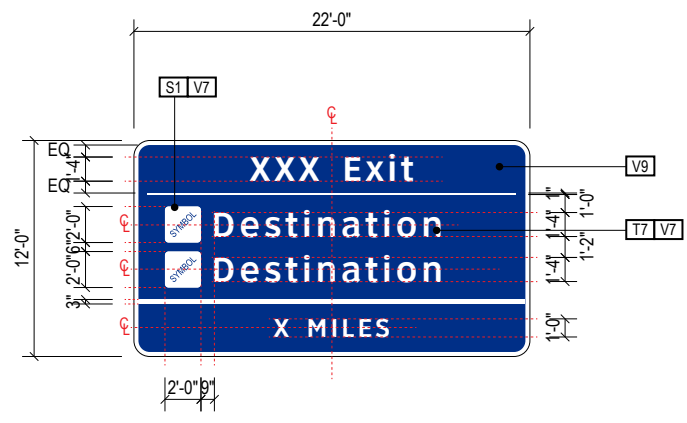
A4 FACE LAYOUT: 4-DR.06 (Typical) Scale: 3/32" = 1'-0"
