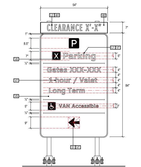
A FACE LAYOUT NTS
