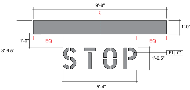
9 STOP PAVEMENT MARKING DETAIL Not To Scale
