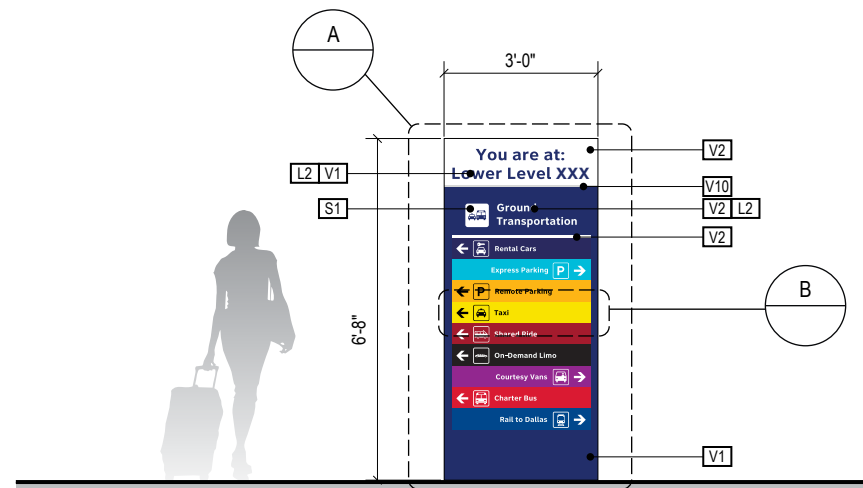
2 ELEVATION - Terminal Exit View
