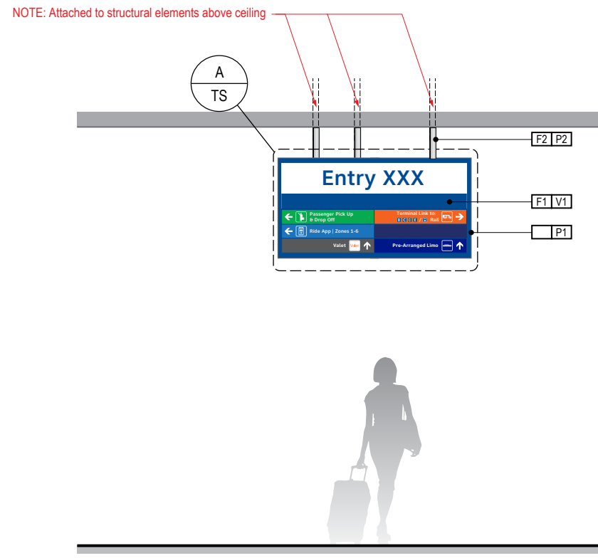
4 ELEVATION (OPPOSITE SIDE) ENTRY VIEW Scale: 1/4" = 1'-0"
