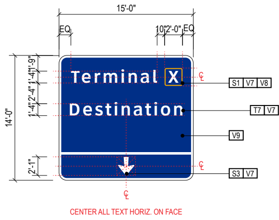
A1 FACE LAYOUT: 4-DR.01 (Typical) Scale: 3/32" = 1'-0" ALIGN
