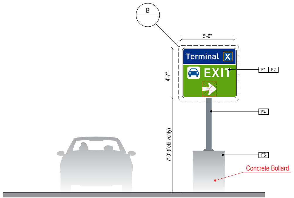
4 ELEVATION w/ Existing Concrete Bollard Scale: 3/16" = 1'-0"
