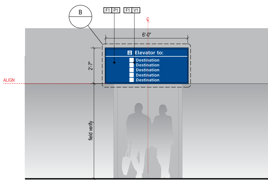
3 ELEVATION - SINGLE ELEVATOR CONDITION Scale: 1/4" = 1'-0"
