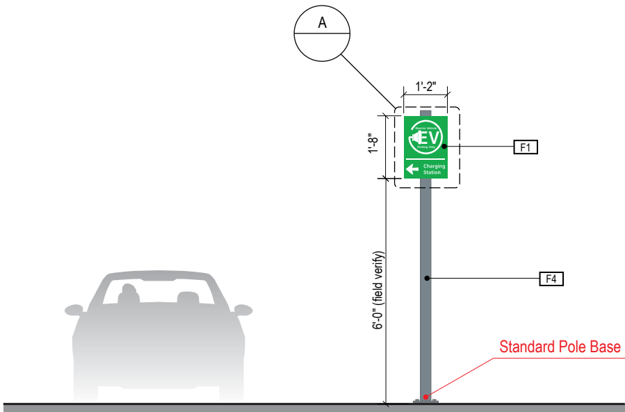
2 ELEVATION w/ Standard Base Scale: NTS
