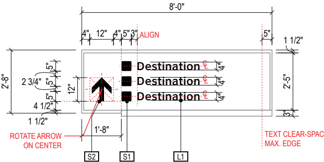
A DETAIL A: Face Layout
