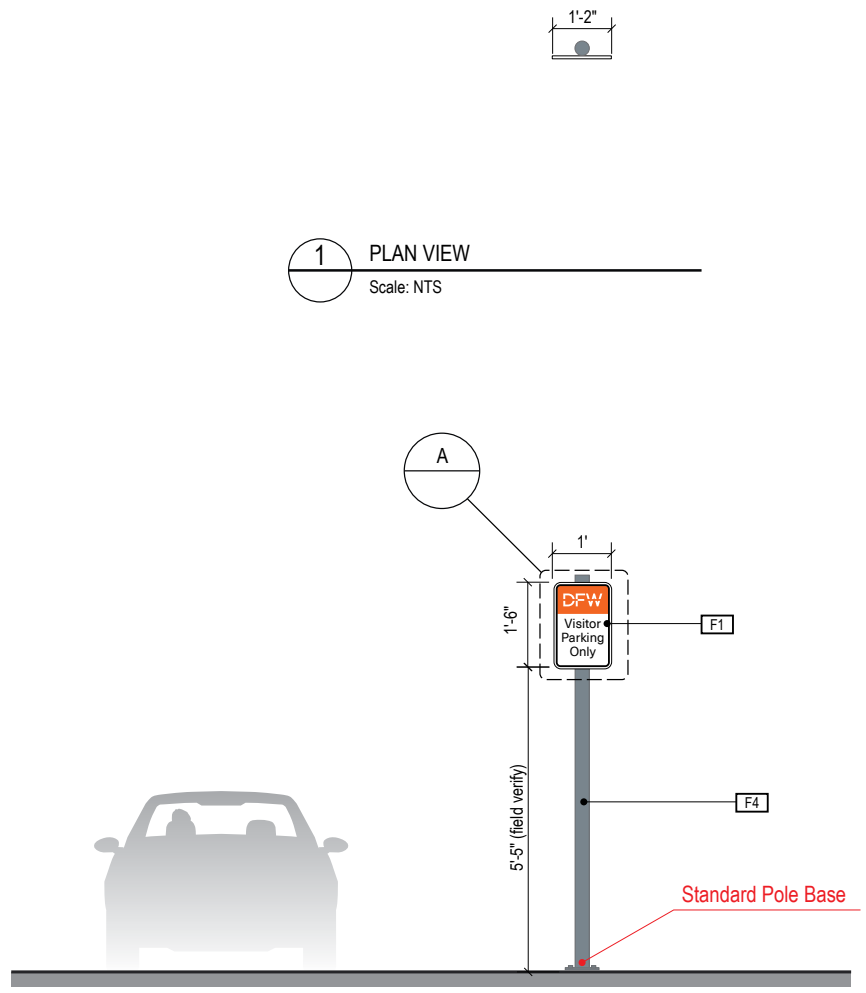
2 ELEVATION w/ Standard Base Scale: NTS
