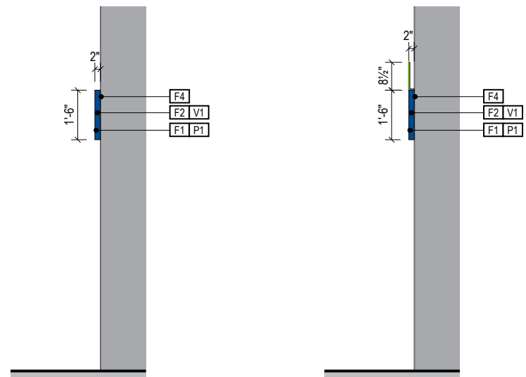
1a END VIEW ELEVATOR Scale: 1/4" = 1'-0"
