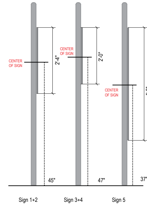
3 END VIEW
