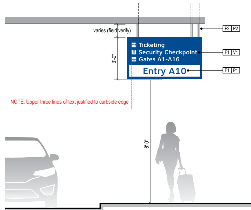
3 ROAD VIEW Scale: 1/4" = 1'-0"
