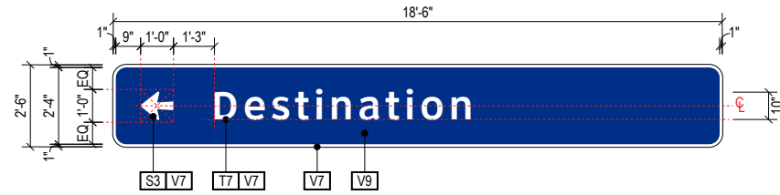
A9 FACE LAYOUT - *Typical Example (C-11-GM04 shown) Scale: 3/16" = 1'-0"
