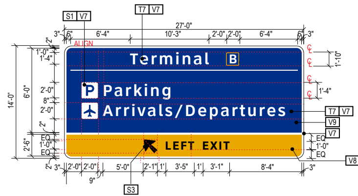
S-NB-3 Vehicular Directional Panel - Two Line Terminal (27'-0" w x 14'-0" h)
