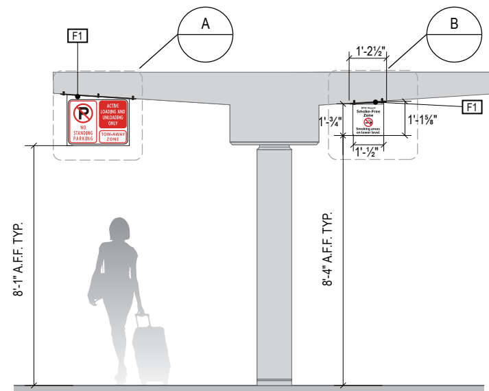
2 ELEVATION (View on Curb) Scale: 1/4" = 1'-0"
