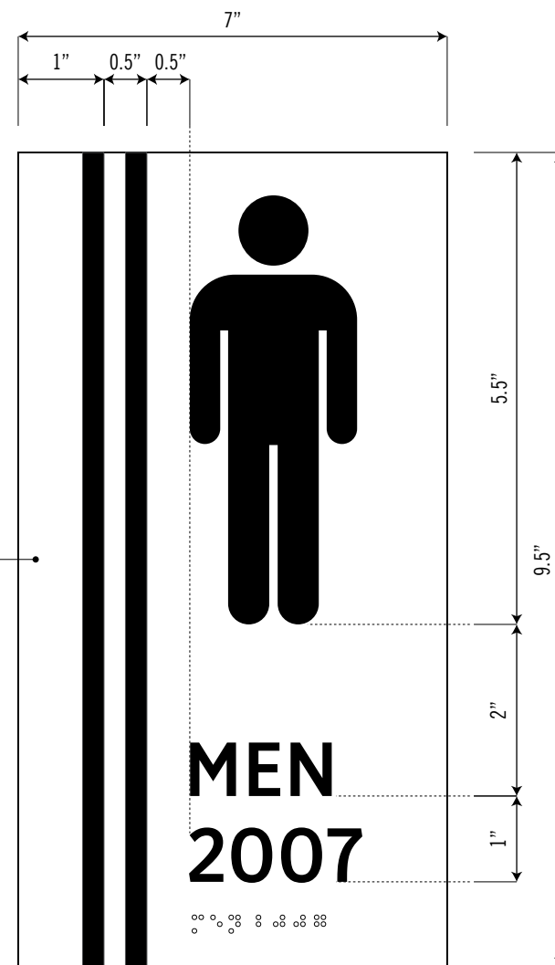
1 Elevation / Half Size Style A
