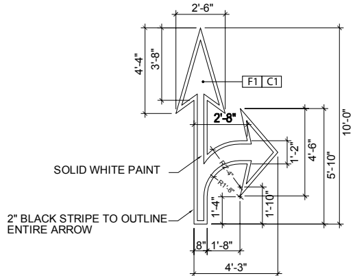
2 STRAIGHT RIGHT ARROW PAVEMENT MARKING DETAIL Not To Scale
