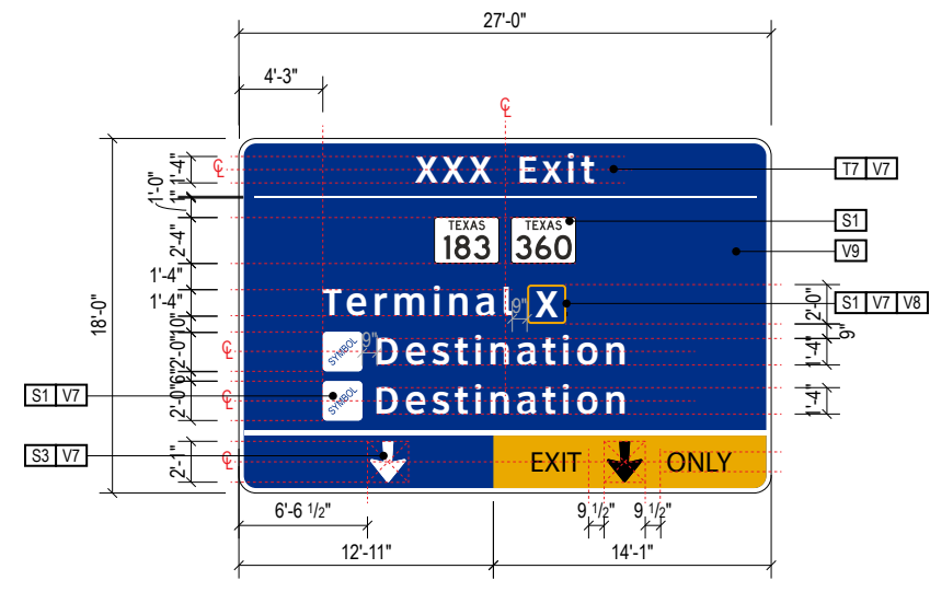
A6 FACE LAYOUT: 4-DR.12 (Typical) Scale: 3/32" = 1'-0"
