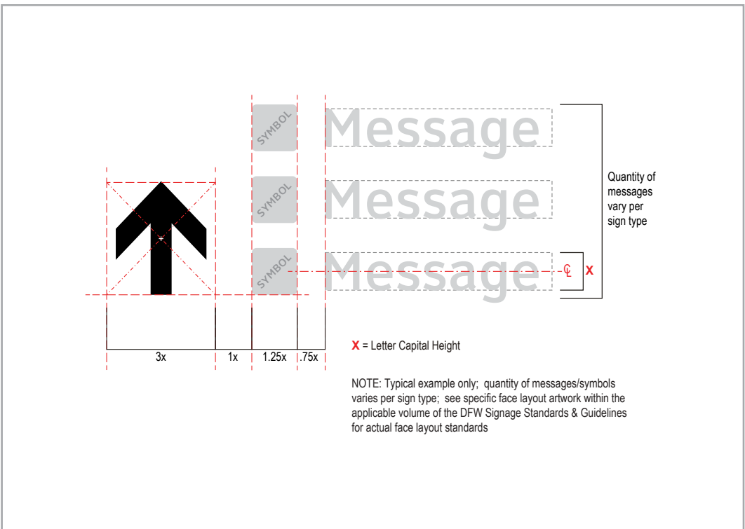
Figure 2.4.1d Wayfinding Arrows: Size Relationships - Pedestrian
