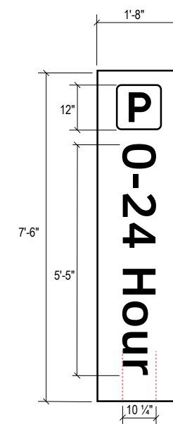
B FACE LAYOUT: D Garage Parking Scale: 1/2" = 1'-0"
