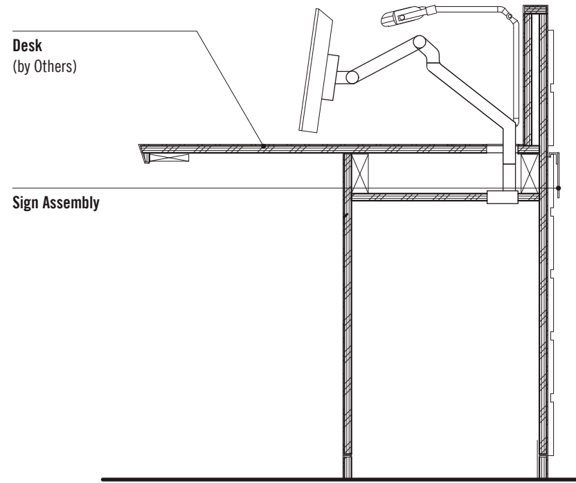
4 Mounting Detail / 3" = 1' - 0"
