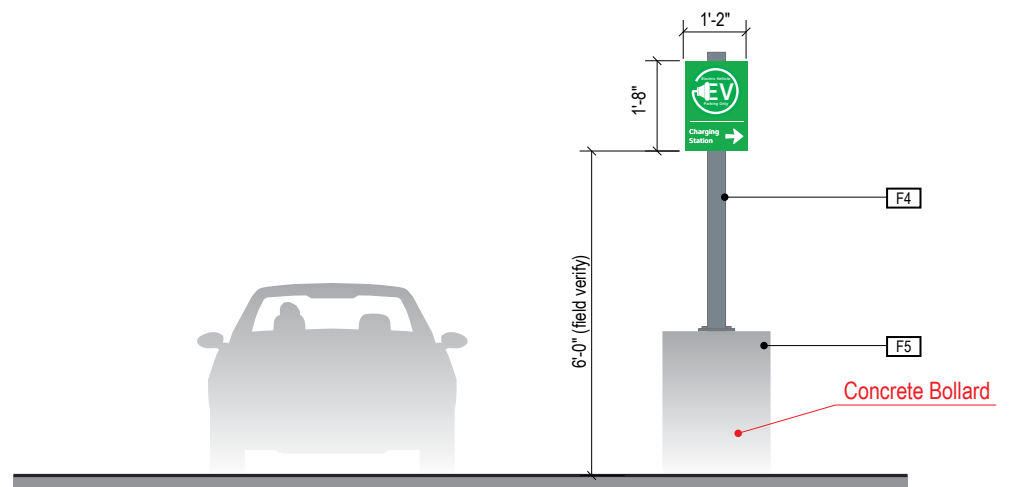
4 ELEVATION w/ Existing Concrete Bollard Scale: NTS
