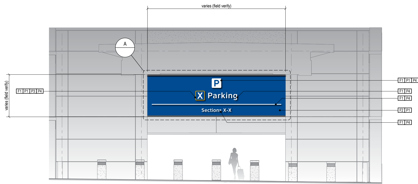
1 ELEVATION (TYPICAL) Scale: 1/8" = 1'-0"
