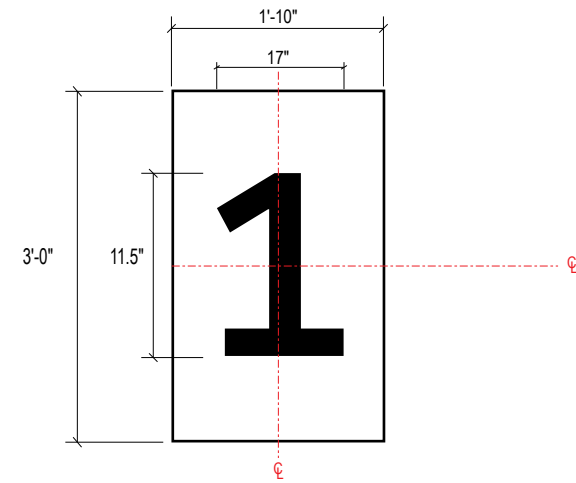
B FACE LAYOUT: Non-Row Sides Scale: 1/2" = 1'-0"
