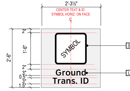
B DETAIL A: Front Face Layout Scale: NTS
