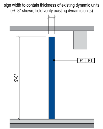
2 SIDE VIEW Scale: 3/16" = 1'-0"
