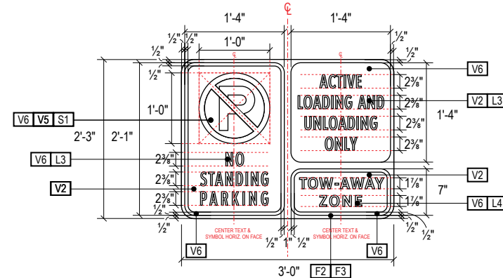
B DETAIL B: Reverse No Parking Face Layout NTS
