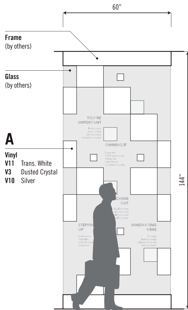
1 Elevation / 3/8" = 1' - 0" Lounge Panel 1, Side A Shown
