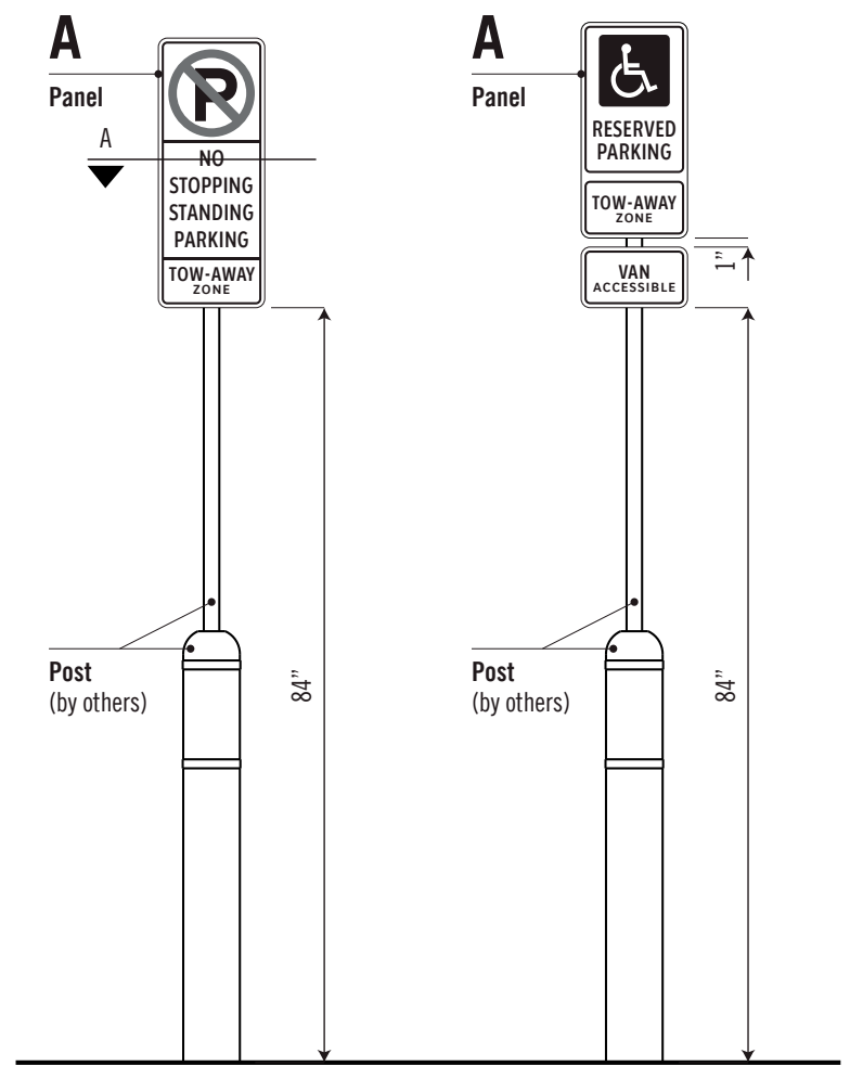
2 Elevation / 1/2" = 1' - 0"
