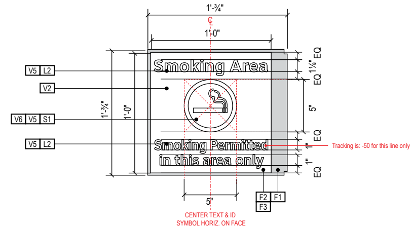
B DETAIL B: Smoking Face Layout NTS
