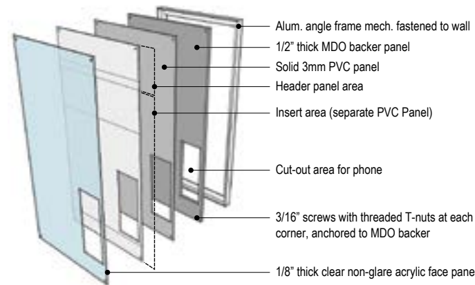
2 PERSPECTIVE (EXPLODED VIEW)
