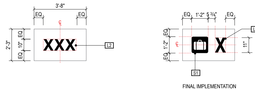
A DETAIL: Face Layout Scale: 1/4" = 1'-0"
