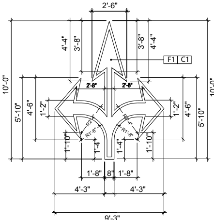
4 STRAIGHT LEFT RIGHT ARROW PAVEMENT MARKING DETAIL Not To Scale
