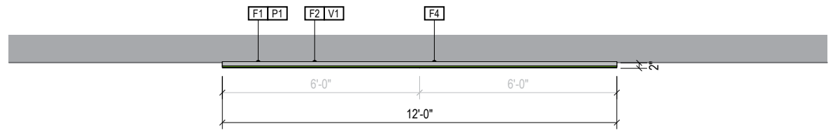
2b PLAN VIEW ENTRY/EXIT DOORS Scale: 1/4" = 1'-0"
