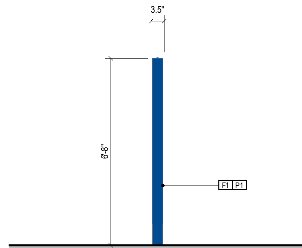
3 SIDE VIEW
