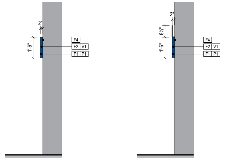
1a END VIEW ELEVATOR Scale: 1/4" = 1'-0" 1b END VIEW ENTRY/EXIT DOORS Scale: 1/4" = 1'-0"
