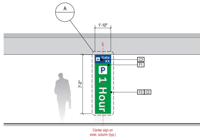
2 ELEVATION: Temp. Parking Scale: 3/16" = 1'-0"
