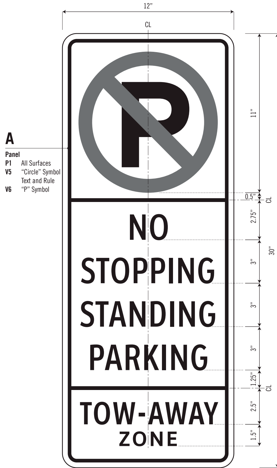
1 Elevation / 3" = 1' - 0"
