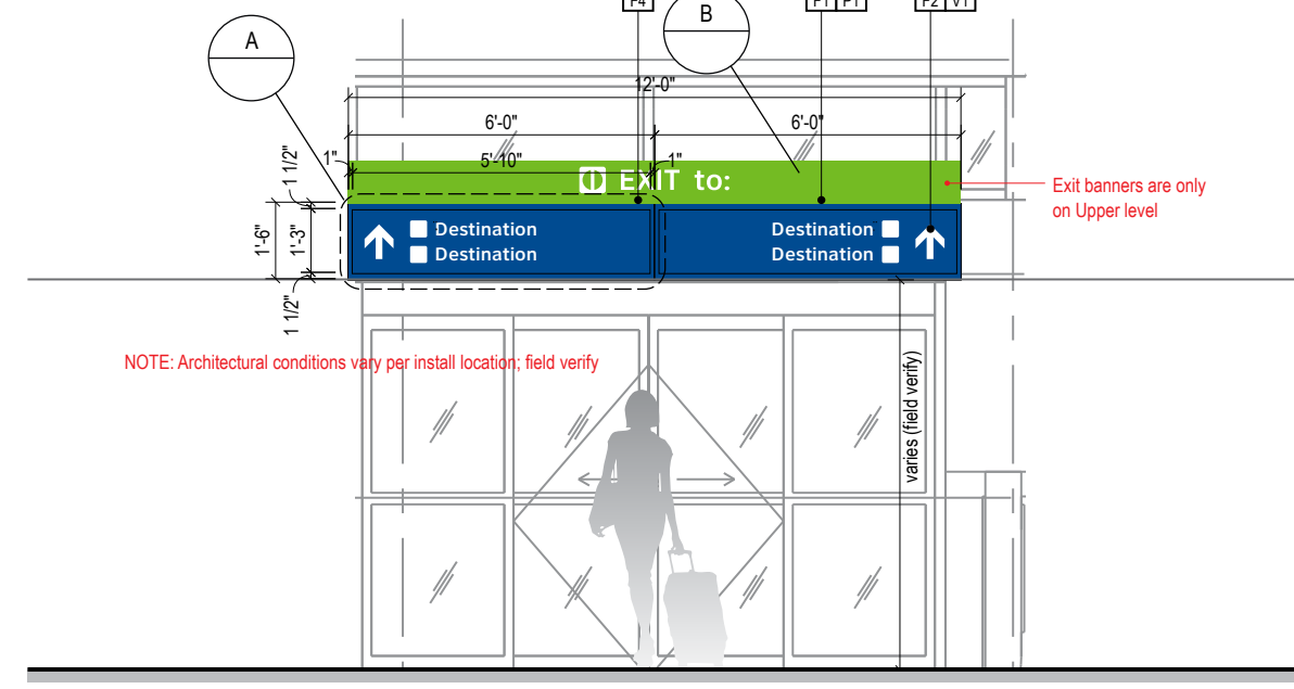
3b ELEVATION ENTRY/EXIT DOORS Scale: 1/4" = 1'-0"
