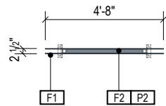
1 PLAN VIEW Scale: 3/16" = 1'-0"
