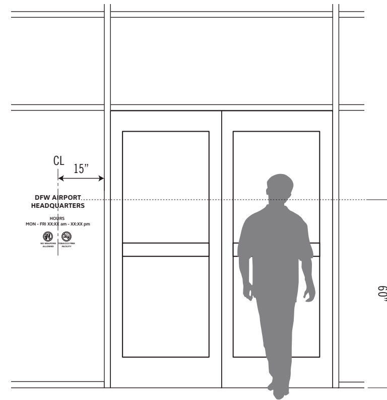
2 Elevation / 3/8" = 1' - 0"
