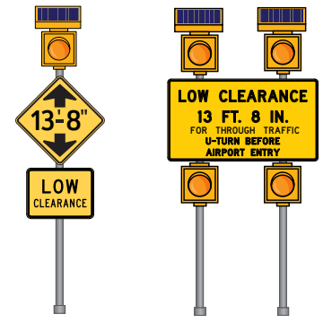
C-14-GM02 Vehicular Int. Prkwy TxDOT Standard Signs - Pole Mount
