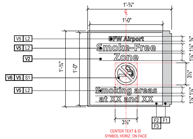
A DETAIL A: No Smoking Face Layout NTS
