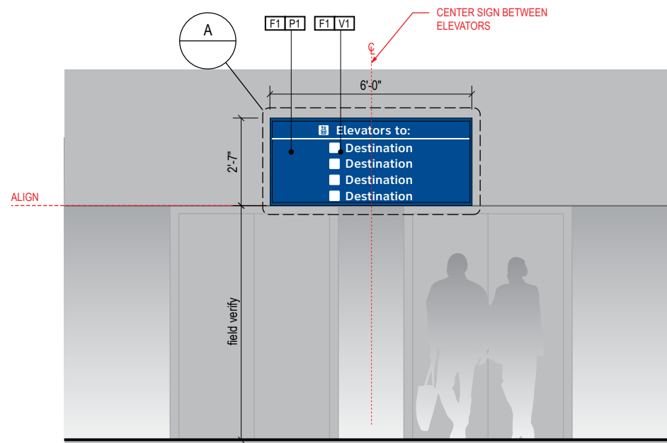
2 ELEVATION - DUAL ELEVATOR CONDITION Scale: 1/4" = 1'-0"
