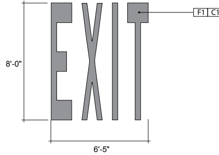
10 EXIT PAVEMENT MARKING DETAIL Not To Scale
