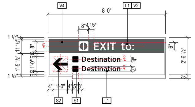
B DETAIL B: Alternate Face Layout
