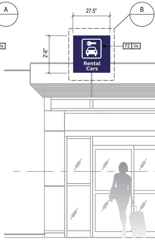
3 ELEVATION (View from Curb) Scale: 1/4" = NTS
