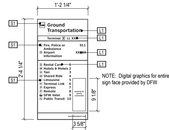
A DETAIL A: Face Layout
