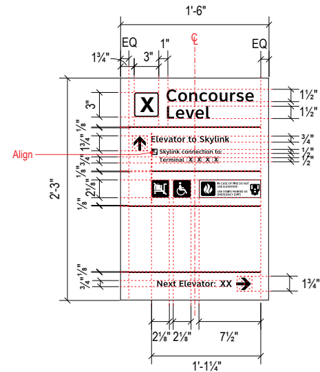
B DETAIL B: Face Layout Scale: 3/4" = 1'-0"
