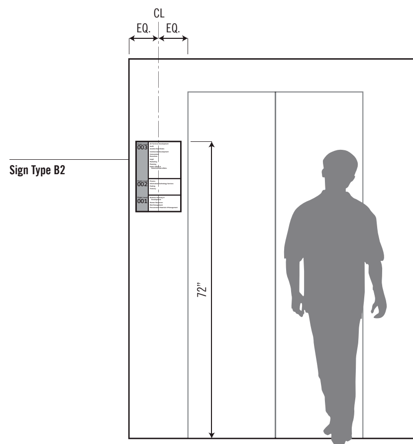
2 Elevation / 1/2" = 1' - 0"
