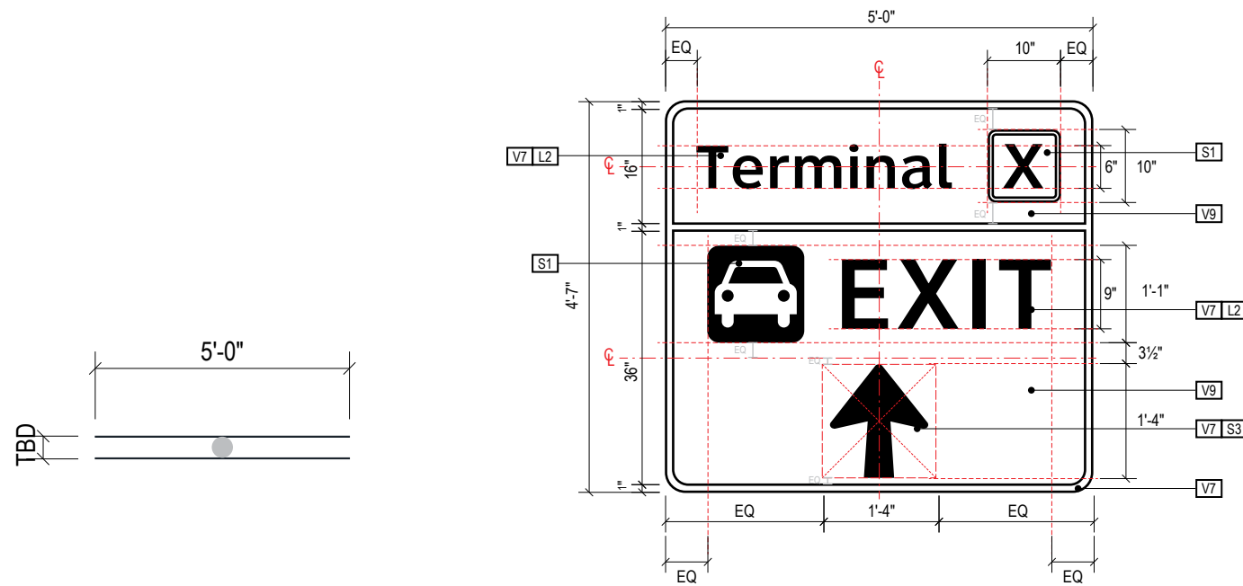
1 PLAN VIEW Scale: 3/16" = 1'-0"
