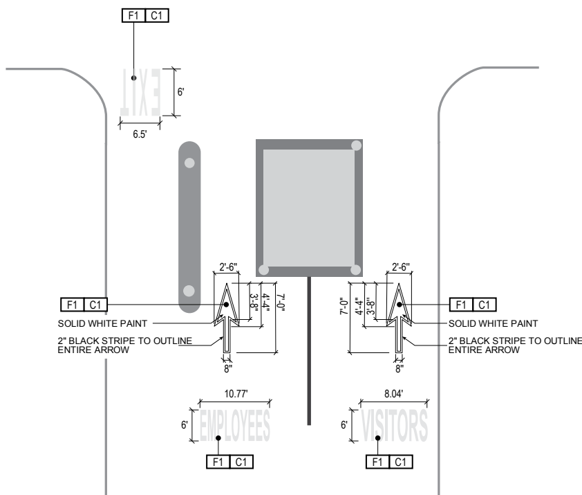
1 PLAN VIEW Scale: NTS
