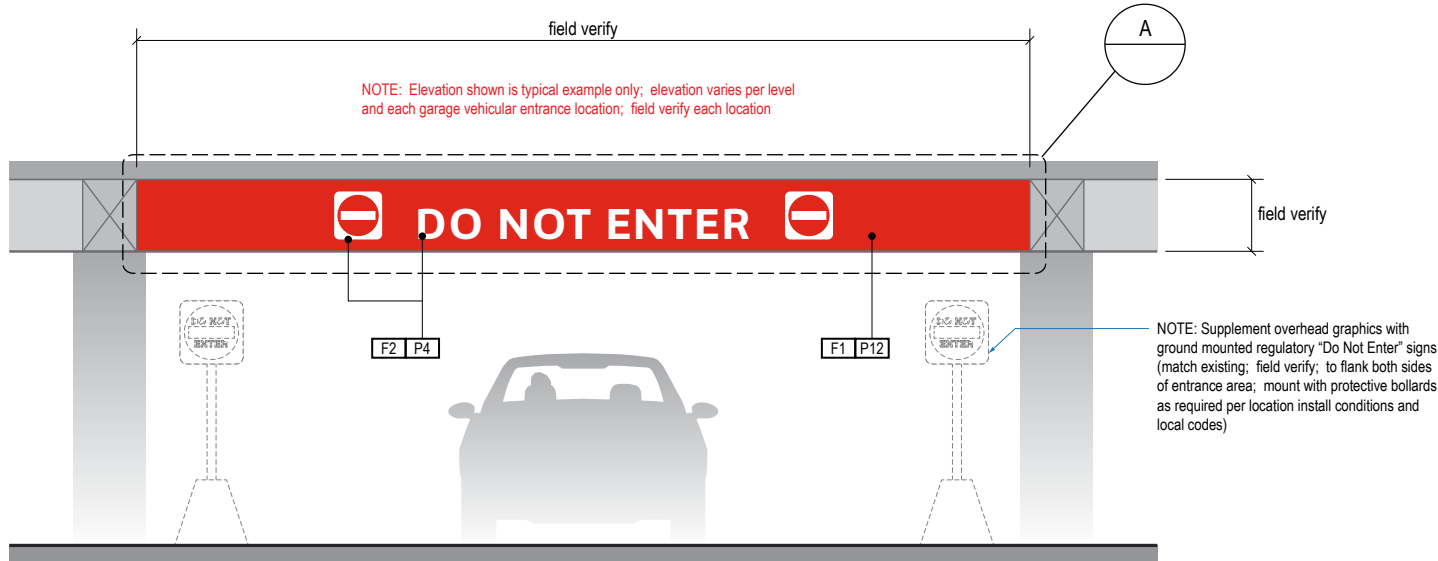
1 ELEVATION: Garage Entrance Area (Typical) Scale: 3/16" = 1'-0"
