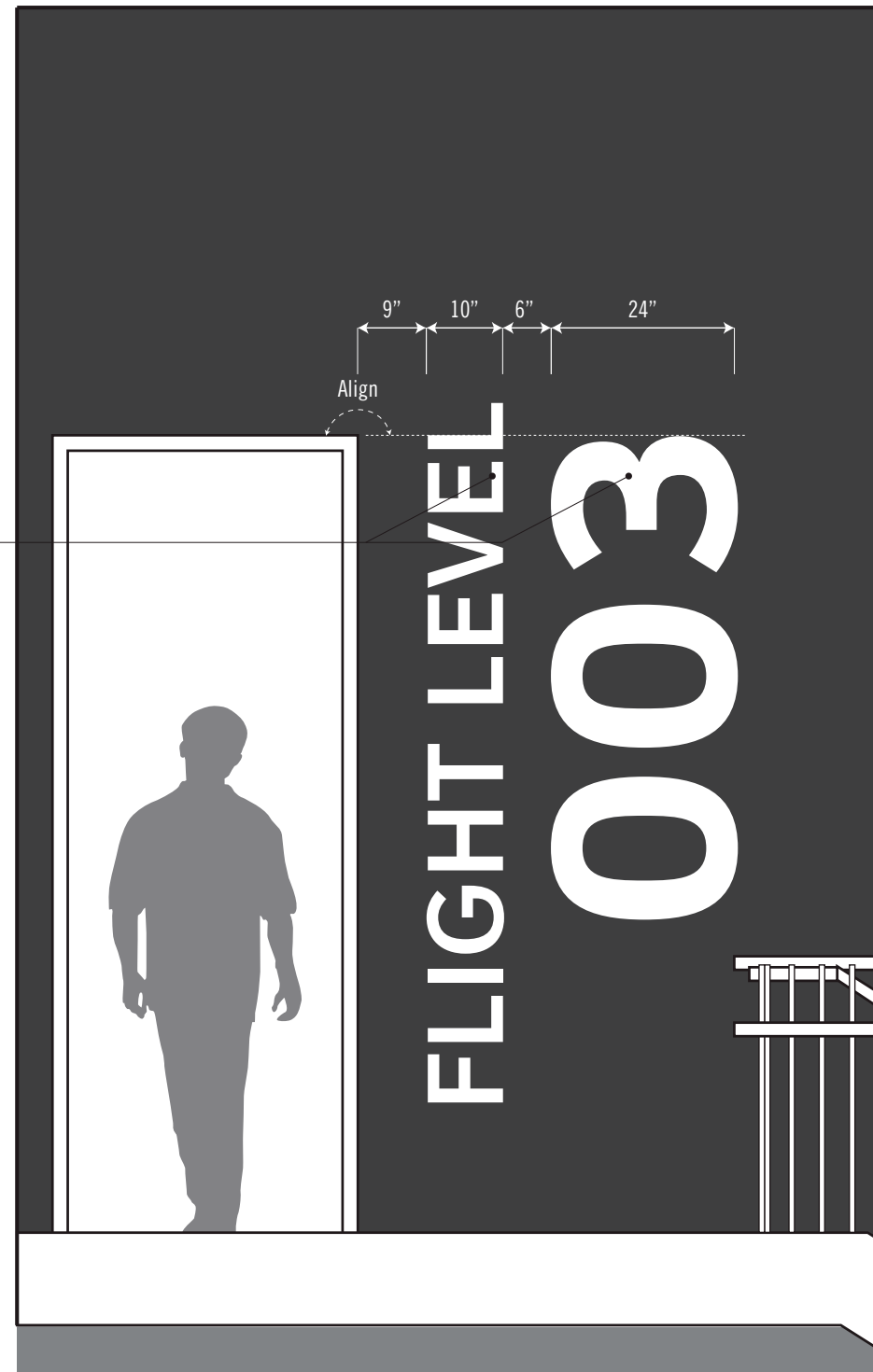
1 Elevation / 1/2" = 1'-0"
