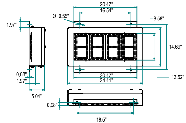
A FACE LAYOUT Digital Component NTS
