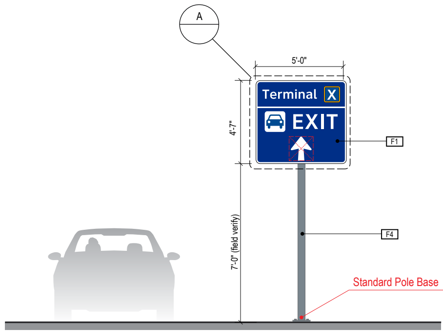
2 ELEVATION w/ Standard Base Scale: 3/16" = 1'-0"
