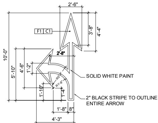
3 STRAIGHT LEFT ARROW PAVEMENT MARKING DETAIL Not To Scale
