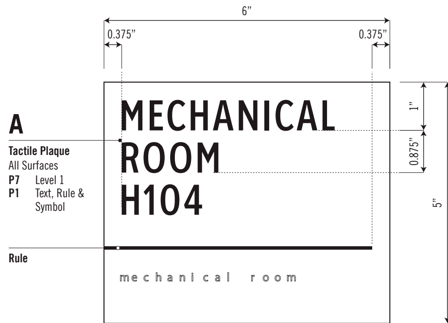
1 Elevation / Half Size
