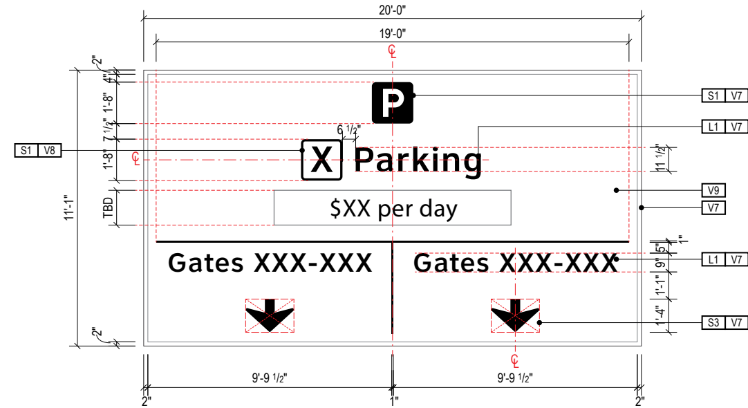
A FACE LAYOUT Scale: 3/16" = 1'-0"
