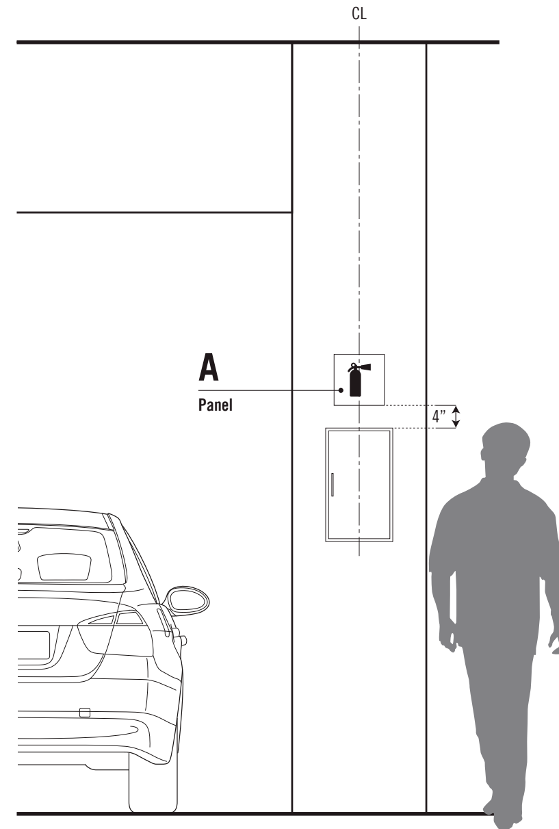
2 Elevation / 1/2" = 1'-0"
