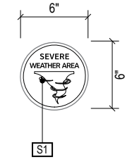
C DETAIL C: Face Layout Scale: 1/2" = 1'-0"
