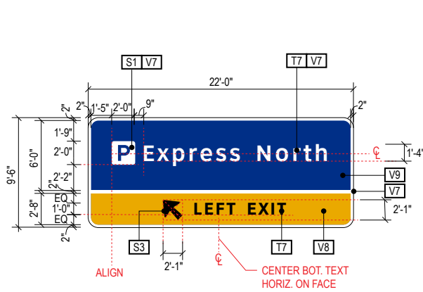
S-NB-1 Vehicular Directional Panel - Cantilever (22'-0" w x 9'-6" h)
