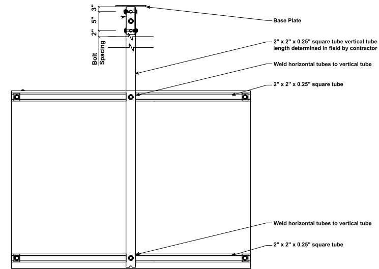
4 Construction Detail NTS
