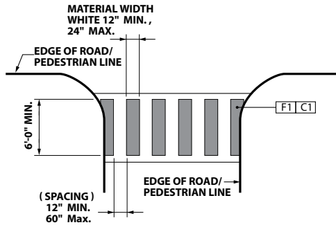
6 STANDARD CROSSWALK PAVEMENT MARKING DETAIL Not To Scale
