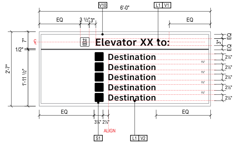
B DETAIL B: Face Layout Scale: 1/2" = 1'-0"
