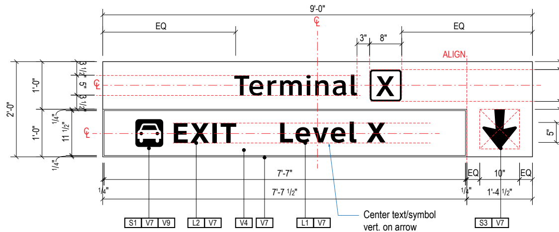
B ALTERNATIVE FACE LAYOUT Scale: 1/2" = 1'-0"
