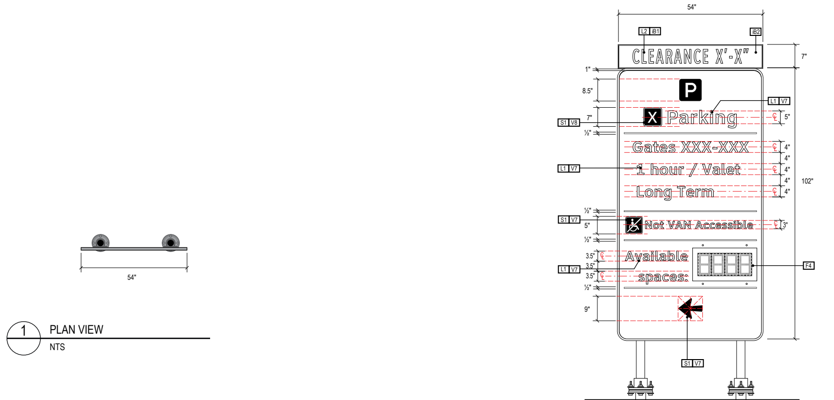
A FACE LAYOUT NTS
