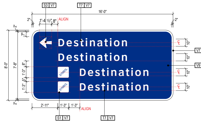
A8 FACE LAYOUT - *Typical Example (C-12-GM03 shown) Scale: 3/16" = 1'-0"
