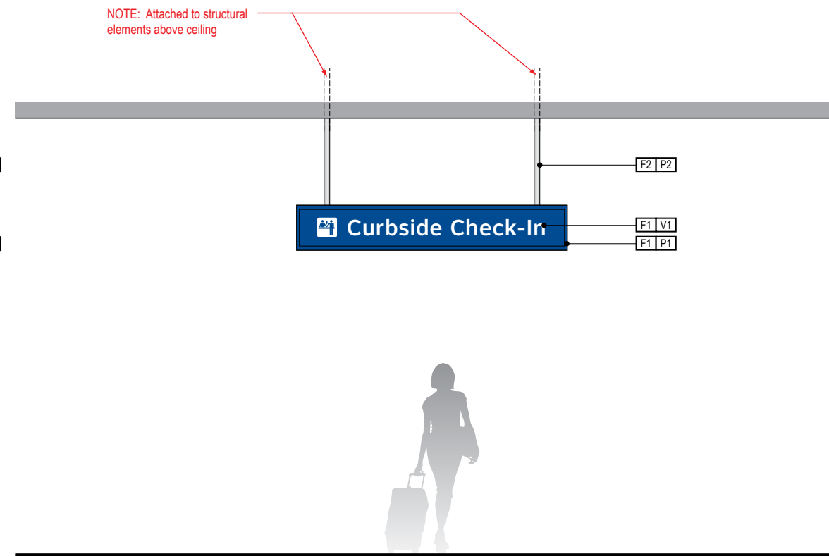
4 ELEVATION (OPPOSITE SIDE) Scale: 1/4" = 1'-0"
