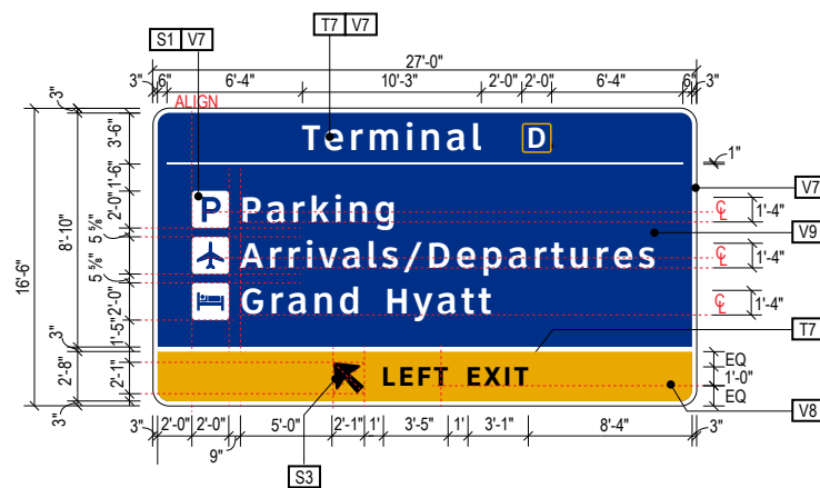
S-NB-2 Vehicular Directional Panel - Three Line Terminal (27'-0" w x 16'-6" h)
