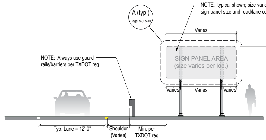
2 ELEVATION (TYPICAL) - Roadside Structure: Small w/ Two Posts Scale: 3/32" = 1'-0"
