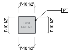
1 PLAN VIEW Scale: 3/16" = 1'-0"
