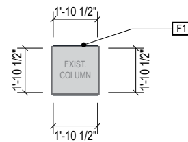
1 PLAN VIEW Scale: 3/16" = 1'-0"
