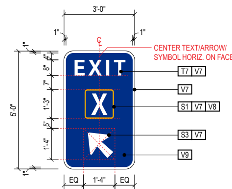
A11 FACE LAYOUT - *Typical Example (IT-NB-22 shown) Scale: 1/4" = 1'-0"
