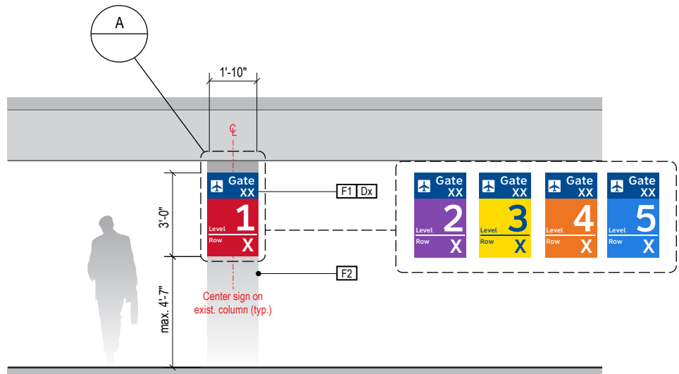
2 ELEVATION: Row Sides Scale: 3/16" = 1'-0"
