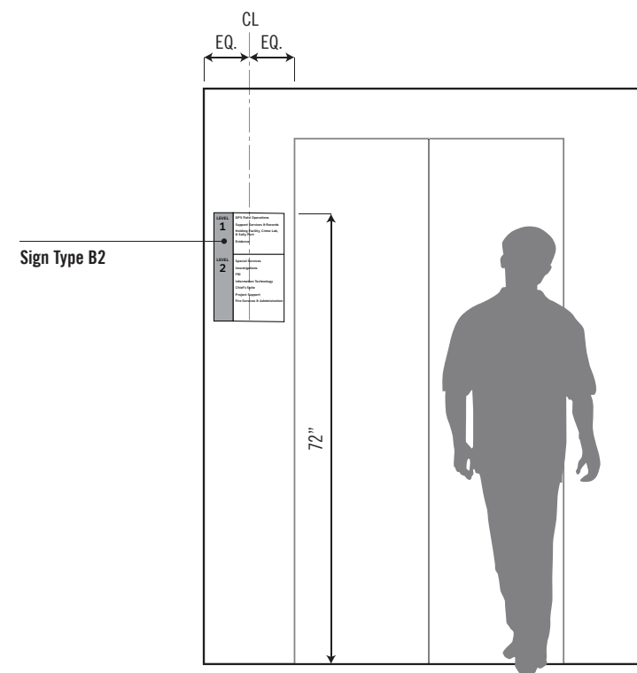
2 ELEVATION - ELEVATOR ENTRANCE VIEW
