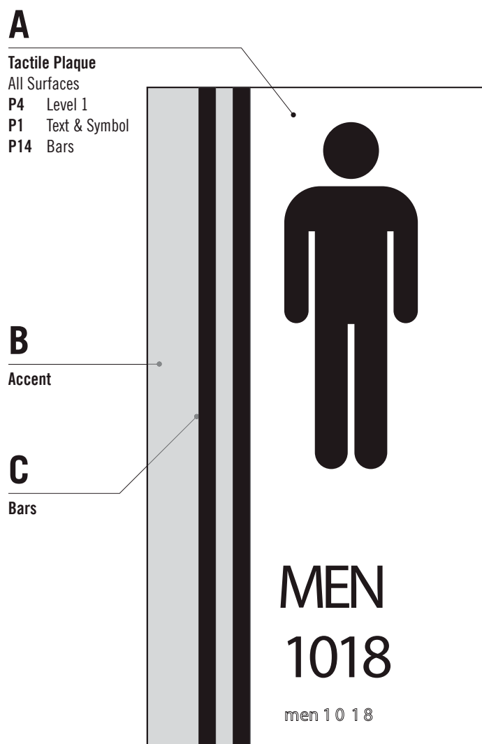
3 Elevation / Half Size Style B
