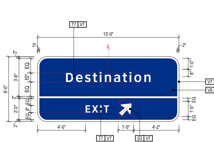
A6 FACE LAYOUT - *Typical Example (S-SB-10 shown) Scale: 3/16" = 1'-0"
