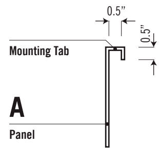
2 Side View / NTS
