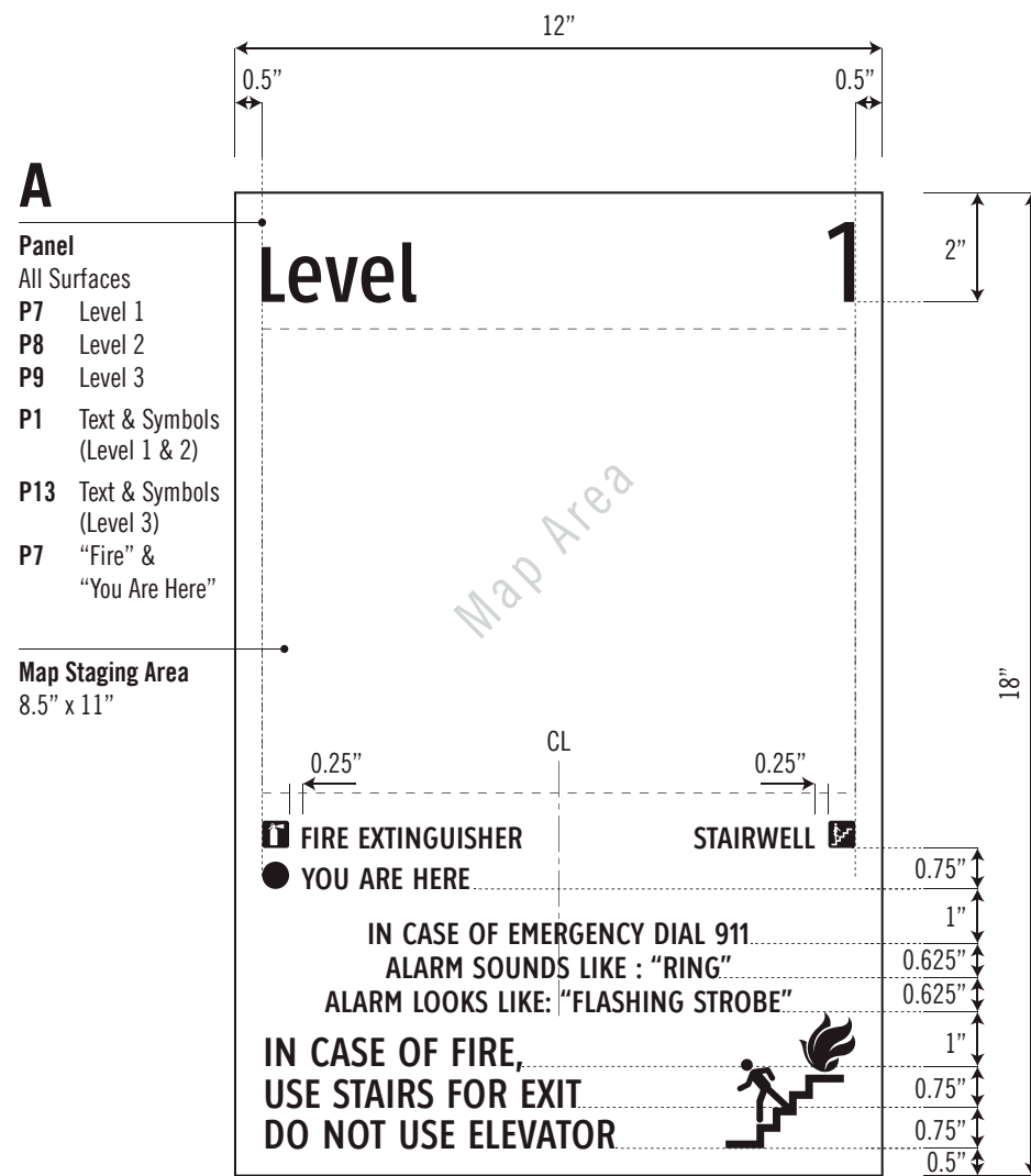
1 Elevation / 3" = 1'-0"
