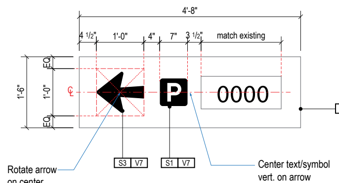
A FACE LAYOUT
