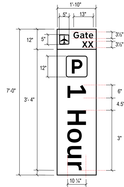
A FACE LAYOUT: Temp. Parking Scale: 1/2" = 1'-0"
