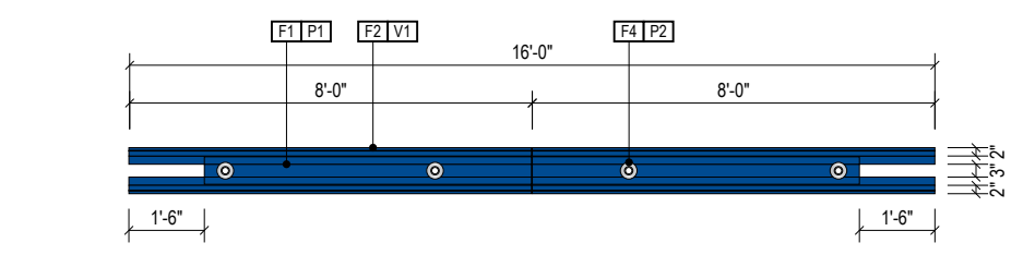
1 PLAN VIEW Scale: 1/4" = 1'-0"
