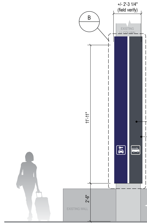
3 ELEVATION (View from Curb) Scale: 1/4" = 1'-0"
