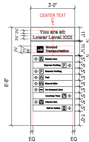
A DETAIL A: Face Layout
