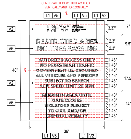
E DETAIL C: Face Layout
