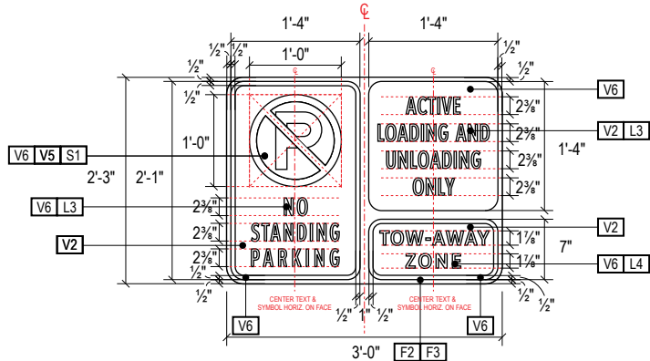
A DETAIL A: No Parking Face Layout NTS
