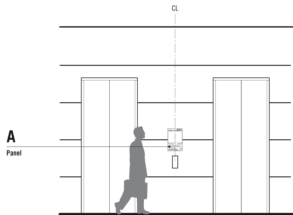
2 Elevation / 1/4" = 1'-0"
