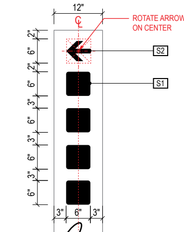
B DETAIL B: Face Layout Scale: 1/2" = 1'-0"
