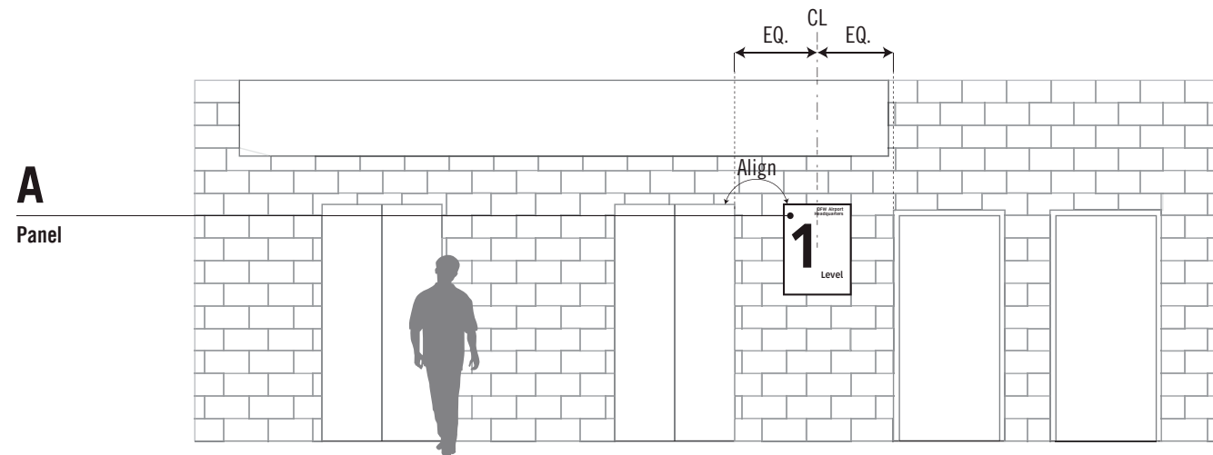
1 Elevation / 3/16" = 1'-0" 1st Floor shown, Typical for 1st and 2nd floor
