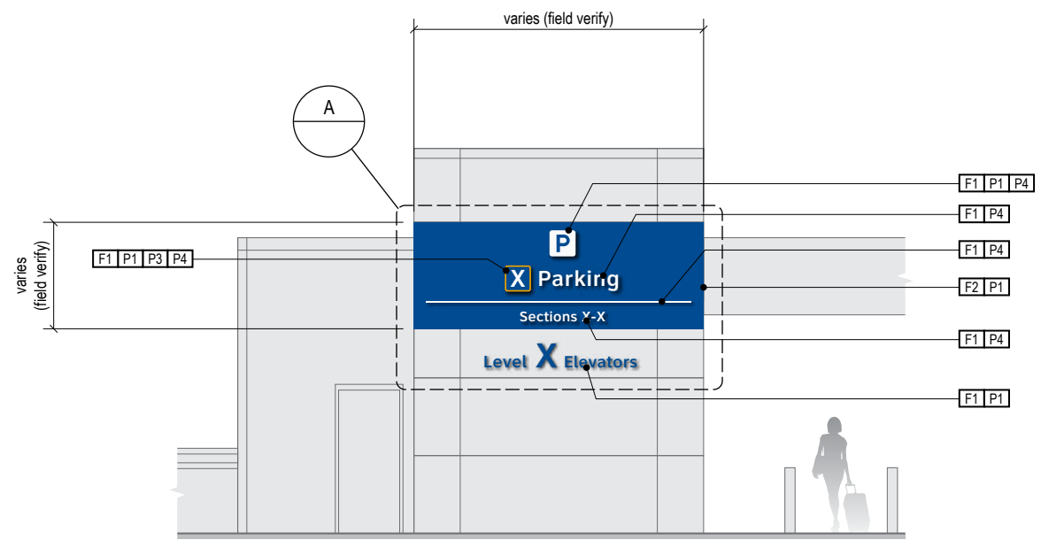
1 ELEVATION (TYPICAL) Scale: 1/8" = 1'-0"
