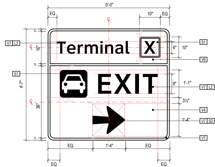
B ALTERNATE FACE LAYOUT OPTION (through garage) Scale: 1/2" = 1'-0"
