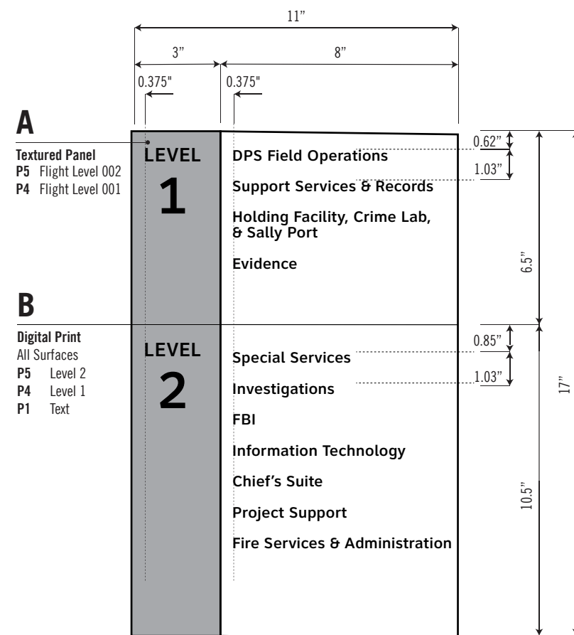
1 ELEVATION - ELEVATOR ENTRANCE VIEW
