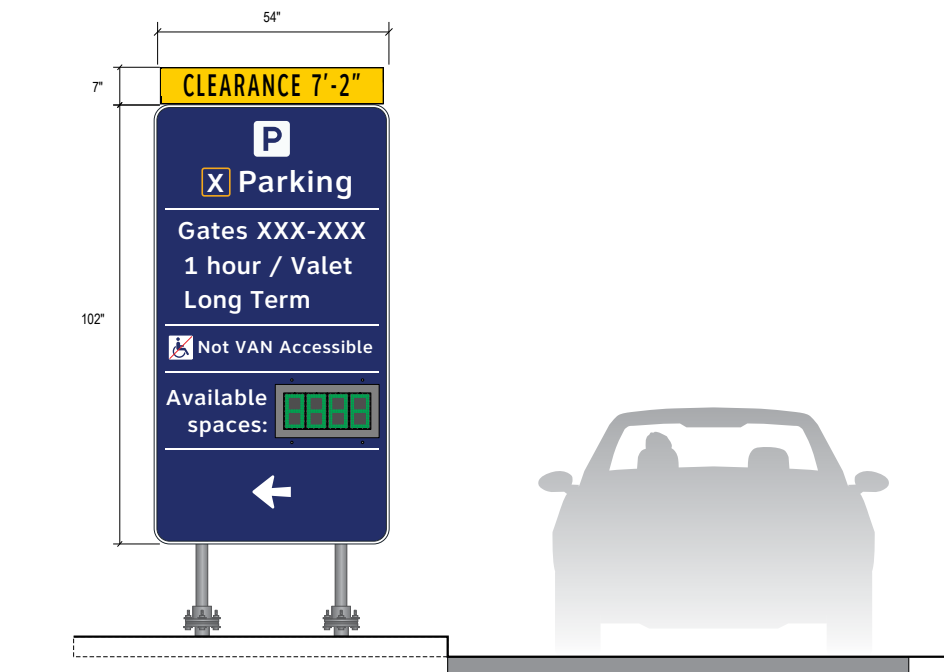
1 ELEVATION: Garage Entrance Area (Typical) NTS
