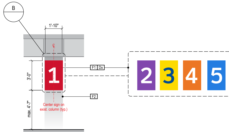
3 Non-Row Sides Scale: 3/16" = 1'-0"
