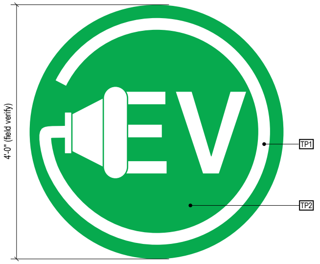
B CHARGING STATION PAVEMENT MARKING Scale: NTS
