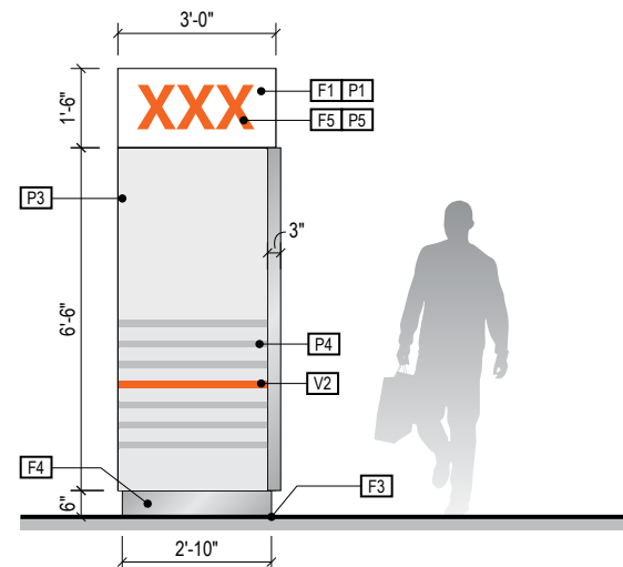
4 ELEVATION (OPPOSITE SIDE) Scale: 1/4" = 1'-0"
