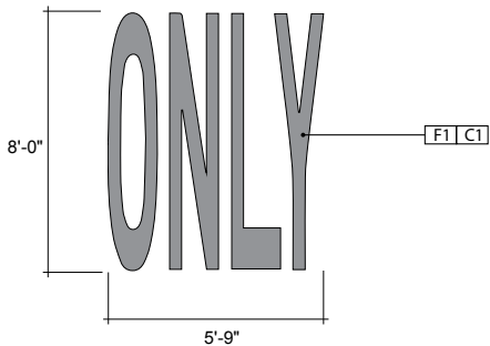
8 ONLY PAVEMENT MARKING DETAIL Not To Scale
