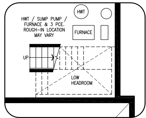
OPT. SERVICE STAIR
