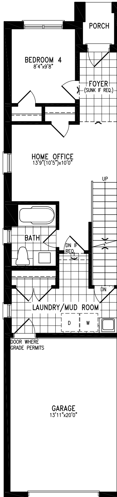
Elevation B GROUND FLOOR
