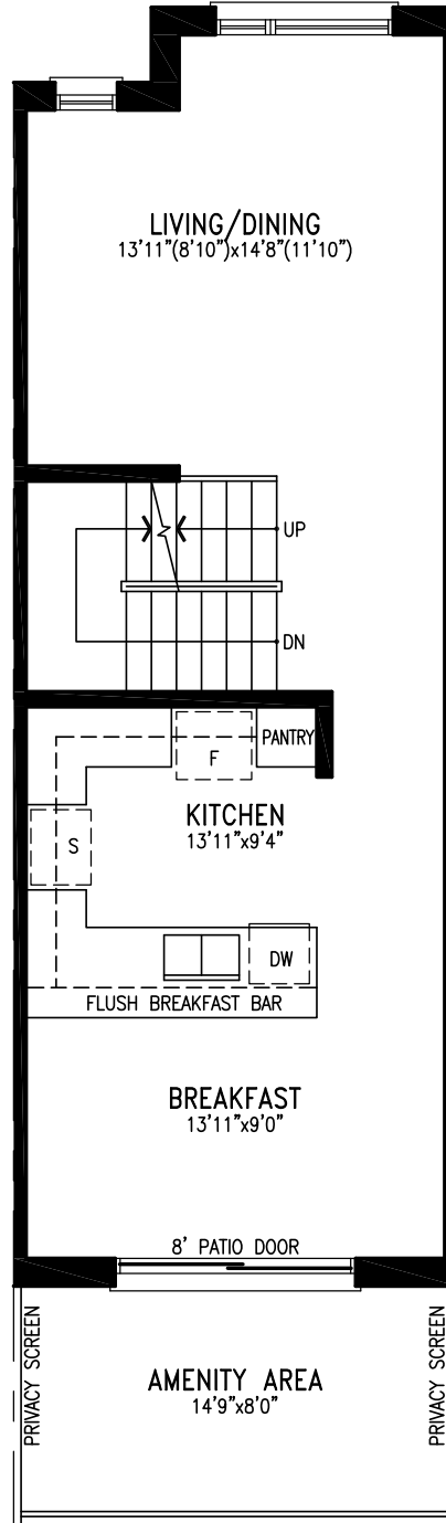
Elevation A MAIN FLOOR
