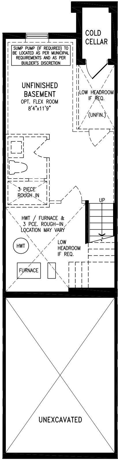
Elevation A BASEMENT
