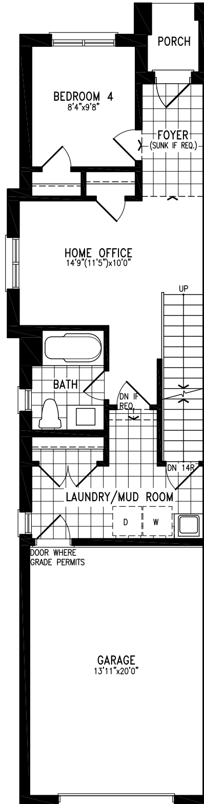
Elevation B GROUND FLOOR SIDE UPGRADE
