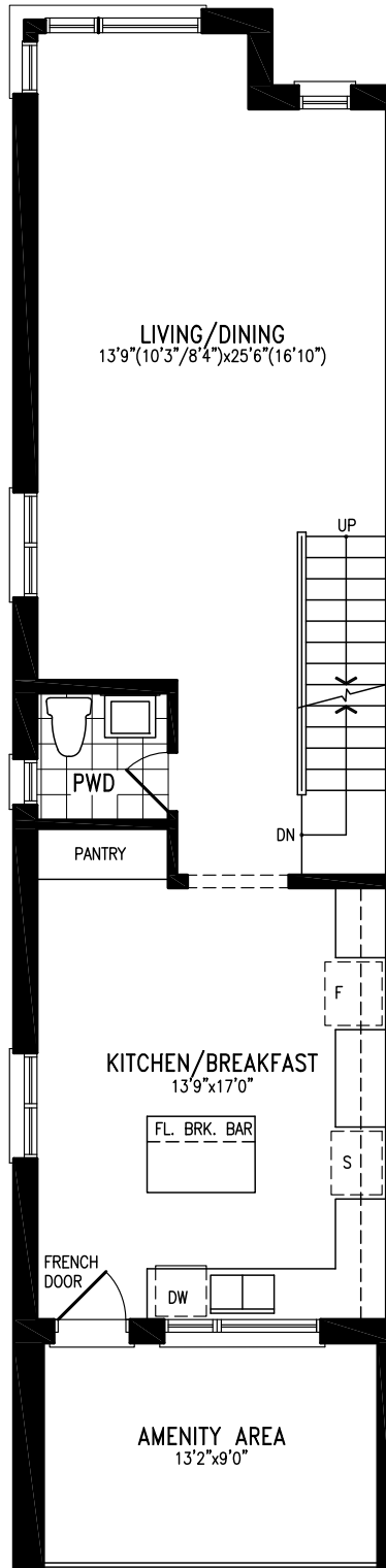
Elevation A MAIN FLOOR
