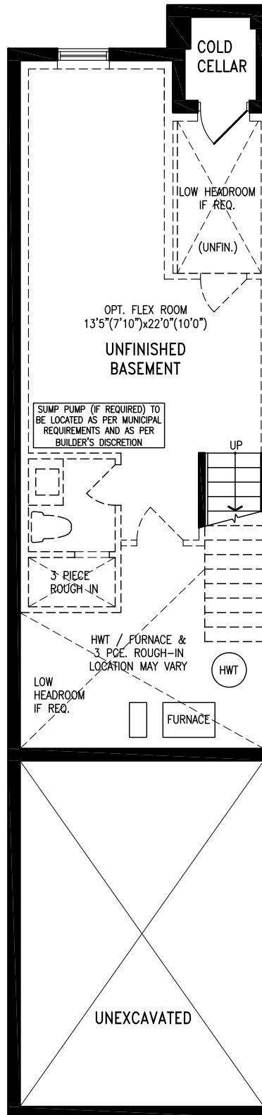
Elevation B BASEMENT
