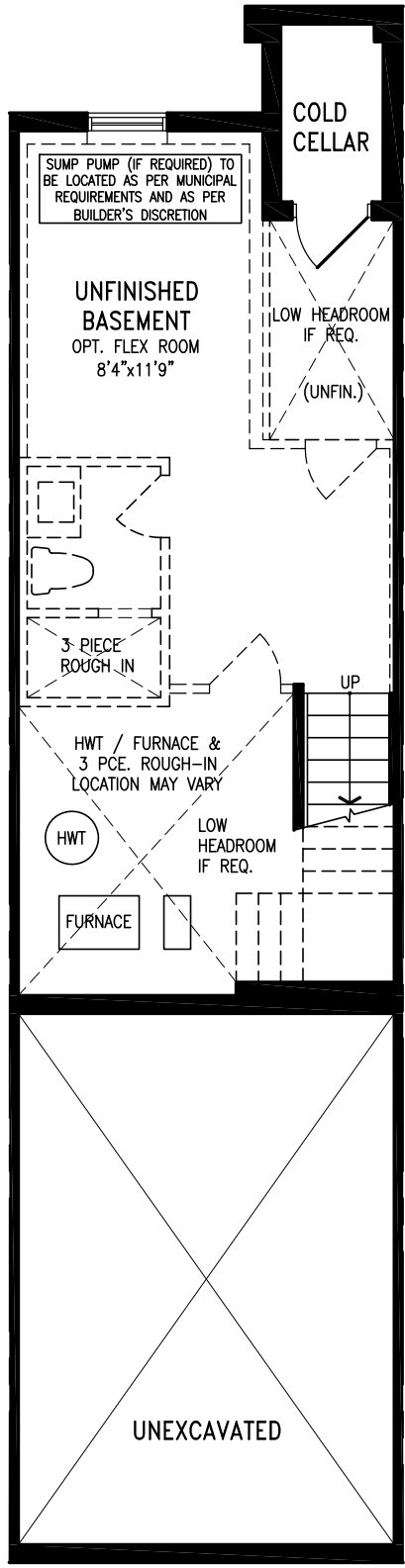
Elevation B BASEMENT
