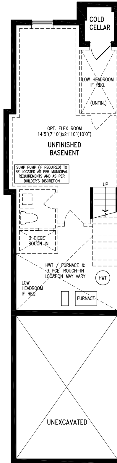
Elevation B BASEMENT SIDE UPGRADE
