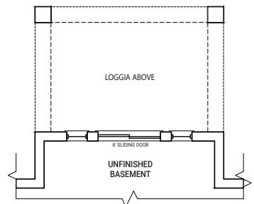
PARTIAL OPT. BASEMENT PLAN W/ OPT. LOGGIA
