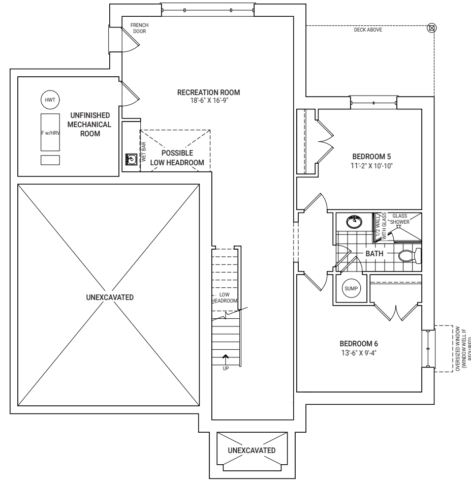
OPT. FINISHED BASEMENT PLAN ELEVATION B
