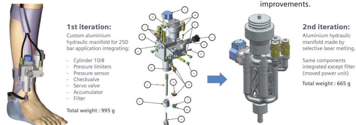
Image provided by HEIA-FR university. First concept for integration of the actuator on an exoskeleton structure and design iterations
