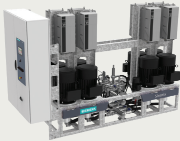
Electric-driven pump unit with frequency converters
