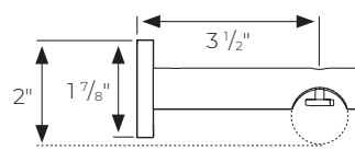
Wall Mount 3 1/2" return PTHMT118400
