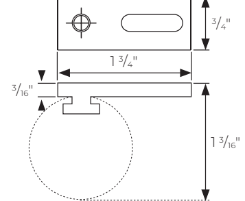
Low-Profile Ceiling Single PTHMT118406
