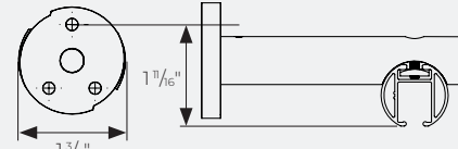
Wall Mount Bracket Mounting Plate
