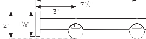
Ceiling Mount Single PTHMT118403
