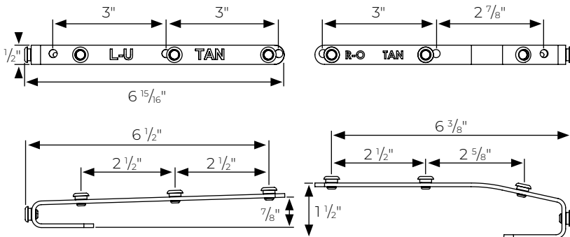
R-TEC Motorized Heavy Duty Traverse ONLY Universal Tandem Master Carrier Arms, Center Draw RTMDTCDTAN (see page 52 for details)
