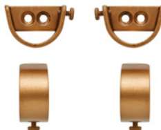
TFCS138MIBK NEW 1⅞" steel inside mount brackets 1¼"H x 1⅞"W backplate, 1"Deep, ¼" thick backplate per bracket (sold in pairs)
