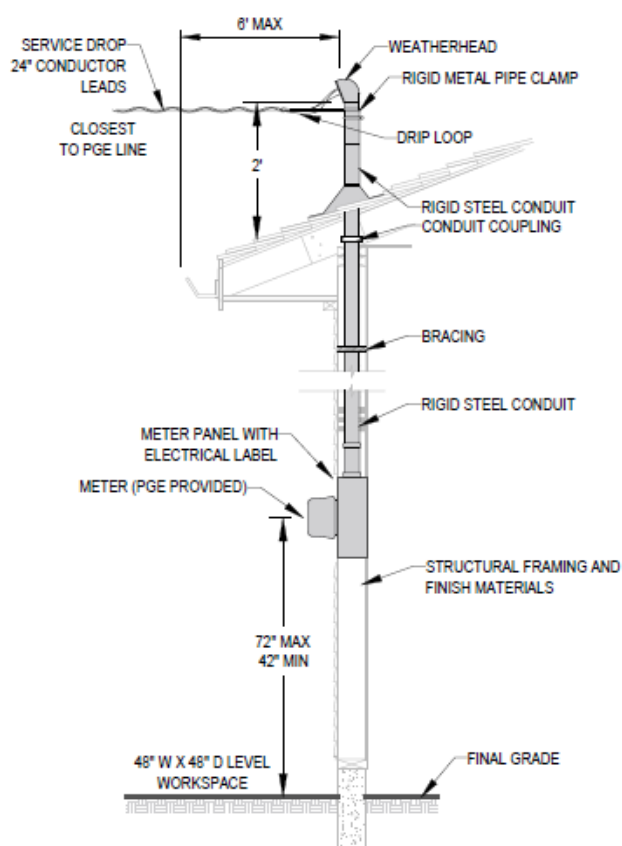
OVERHEAD FLUSH MOUNT METERING UNSUPPORTED - MAST HEIGHT 24"
