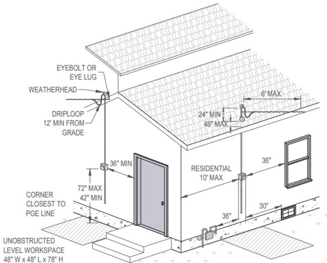
Figure 27. Metering Equipment for Overhead Service (STD-D-2226)
