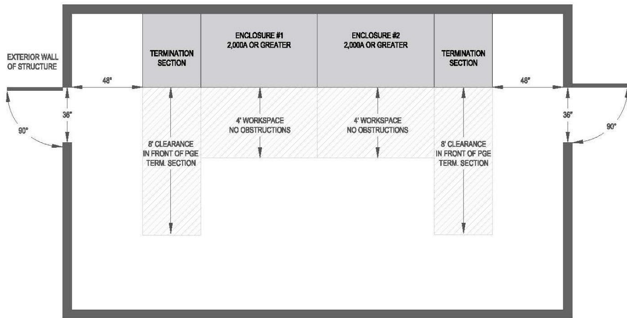
Figure 126. Two-Enclosure Room with Two Doors, 2000 A or Greater
