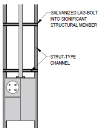
Figure 67. Overhead Service with Service Mast (STD-D-6023)
