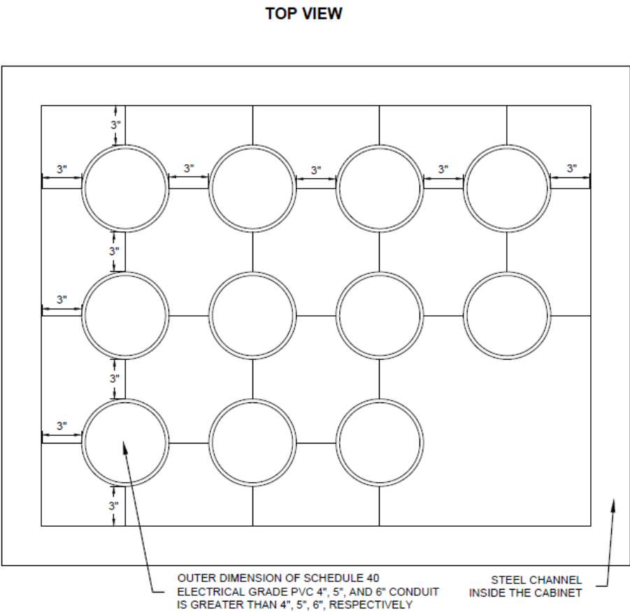
Figure 48. PGE’s Required Separation of Conduit in Customer Gear (STD-D-3121)
