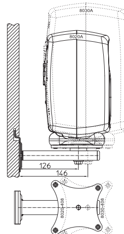
8020 and 8030/8130 on short slatwall bracket.
