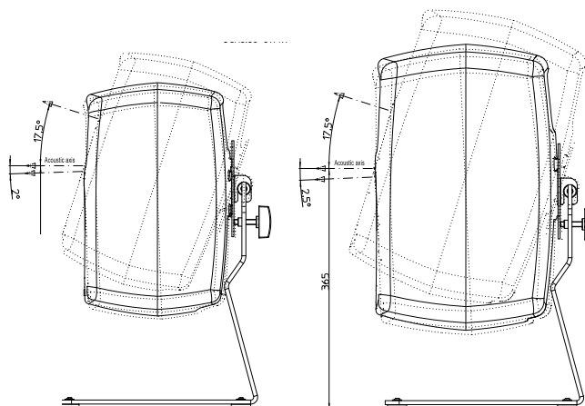
L-shape stand 8000-325B and 8351
