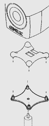
Stand plate and Iso-Pod assembly.
