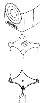
Stand plate and Iso-Pod assembly.
