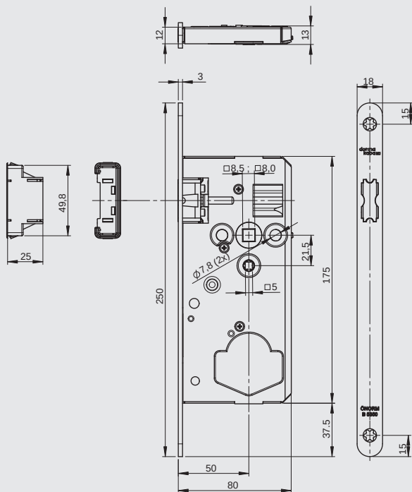
solo/MAF/FA/SB30/R/50/UG/8/NR/250.18.3
