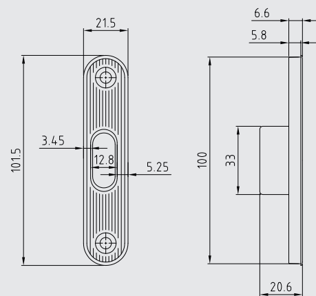
134/SB/BO/VS/TO/Stumpf/20/DS
