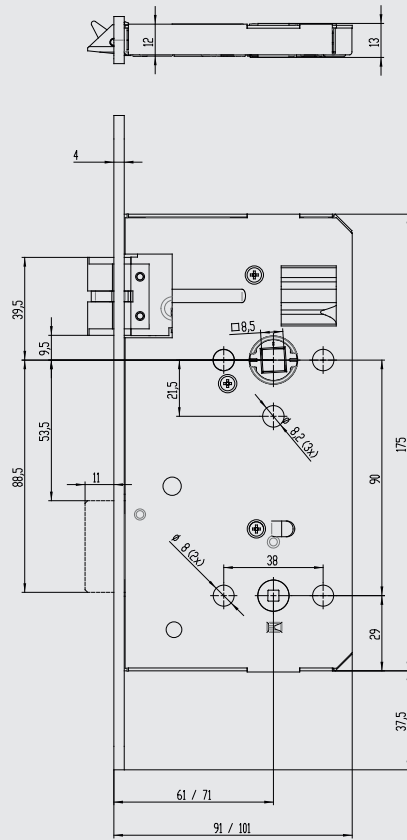
127/WC/KF/R/60 (70)/90/8,5/DS/250.18.4/x
