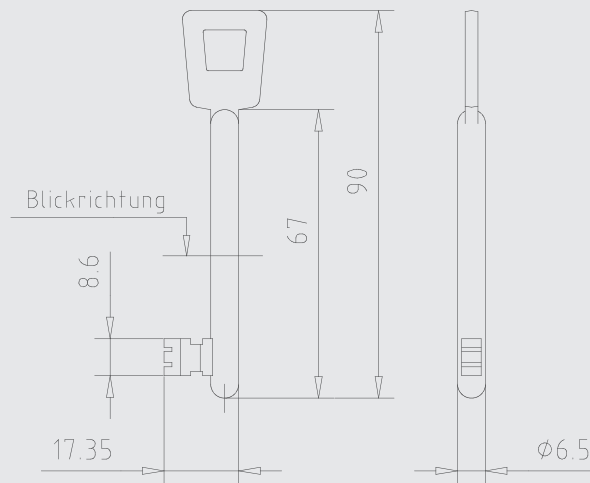
KBSL/* Keilbartschlüssel
