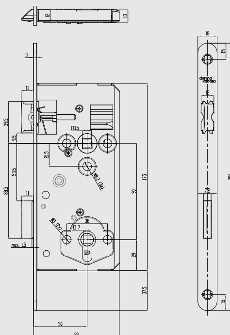
ergo/WC/R/50/90/8,5/DS (SWM)/250.18.3
