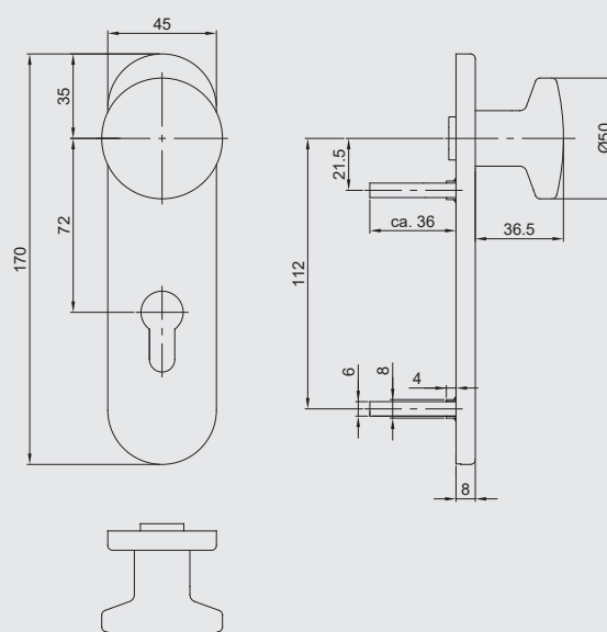
KURZSCHILD+KN/PZ72/MOD1.1/NR
