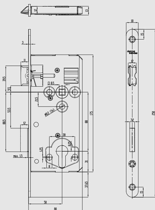
ergo/PZ/R/50/88/8,5/DS (SWM)/250.18.3
