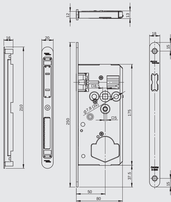
solo/MAF/FA/SB12/R/50/UG/8/NR/250.18.3
