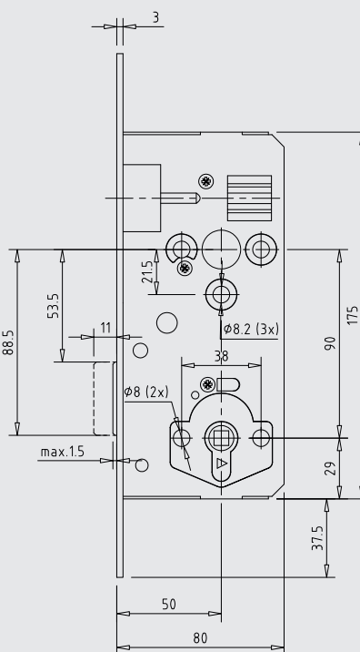
121/WC/R/50/UG/DS/250.18.3/RI
