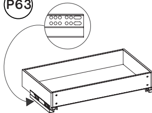
Drawer Box (47cm deep shelf) 101.124.13, 101.124.14
