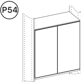
Doors 101.120.xx, 101.121.xx
