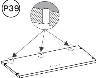
Middle and bottom board 101.142.xx, 101.146.xx
