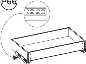
Drawer Box (47cm deep shelf) 101.124.03, 101.124.04
