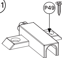
Adapter with regulation 901.100.01
