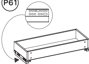
Drawer Box (34cm deep shelf) 101.124.10, 101.124.11
