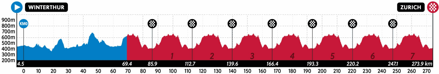
COURSE PROFILE MEN ELITE ROAD RACE Distance : 273.9km (+ 4.5 km) | Total Elevation : 4 470m
