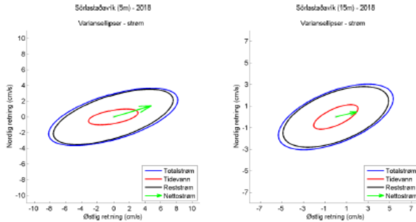
Figure 2. Variance ellipse for total current, tidal current and residual current at 5 and 15 meter. The ellipse shows the size of one standard deviation of the variance, both in direction and size. The blue curve shows the variance ellipse of the total flow and the red curve shows the variance ellipse of the tidal component. The black variance ellipse shows the residual current, ie. the current that cannot be explained by the tide. The results are estimated from current data from the measurement period 14.09.2018-19.10.2018. The green arrow shows net current direction.
