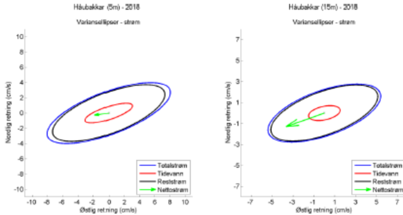
Figure 2. Variance ellipse for total current, tidal current and residual current at 5 and 15 meters. The ellipse shows the size of one standard deviation of the variance, both in direction and size. The blue curve shows the variance ellipse of the total flow and the red curve shows the variance ellipse of the tidal component. The black variance ellipse shows the residual current, ie the current that cannot be explained by the tide. The results are estimated from current data from the measurement period 14.09.2018-19.10.2018. The green arrow shows net current direction.
