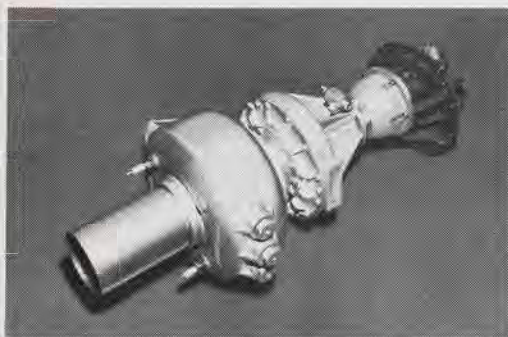
Gene's 1,000 hp, axial-flow turbine develops 1,030 ft. lbs. of torque at stall; 730 ft. lbs. at 7200 rpm.
