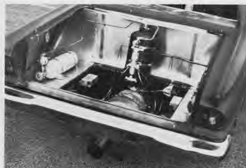
Gene's complete turbine power installation is simple, lightweight. There's nothing under the hood. All weight is over the rear wheels — where it's needed.
