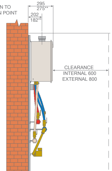
Side view wall mounting
