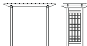
6'W x 7'-7"H 796122
