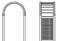
4'W x 8'-1 \frac{1}{4} "H 796101A
