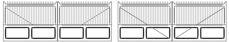
Straight with Recessed Panel Bottom 6'H x 16'W
