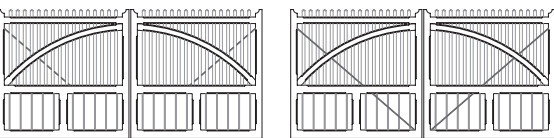
Straight with Arch Brace and Board Panel Bottom 6'H x 12'W
