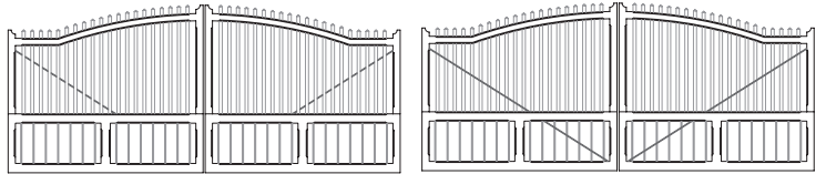
Annisquam Arch with Board Panel Bottom 6'H x 16'W
