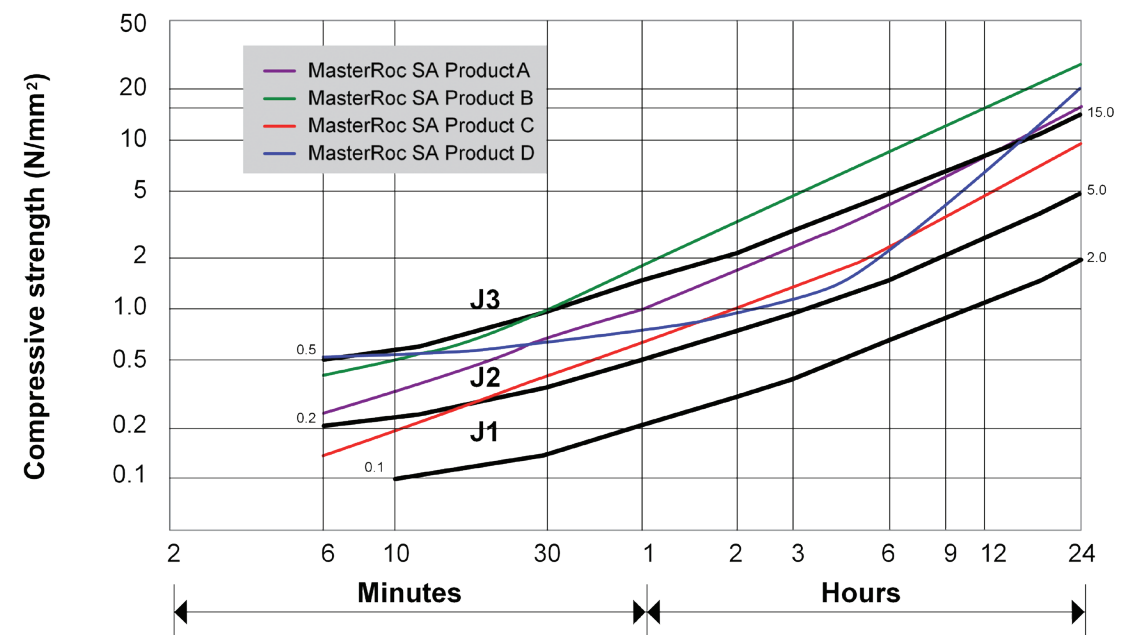
Recorded compressive strength developments by selected alkali-free set accelerators in comparison with J1, J2 and J3 standard requirements based on the Austrian Guideline for sprayed concrete
