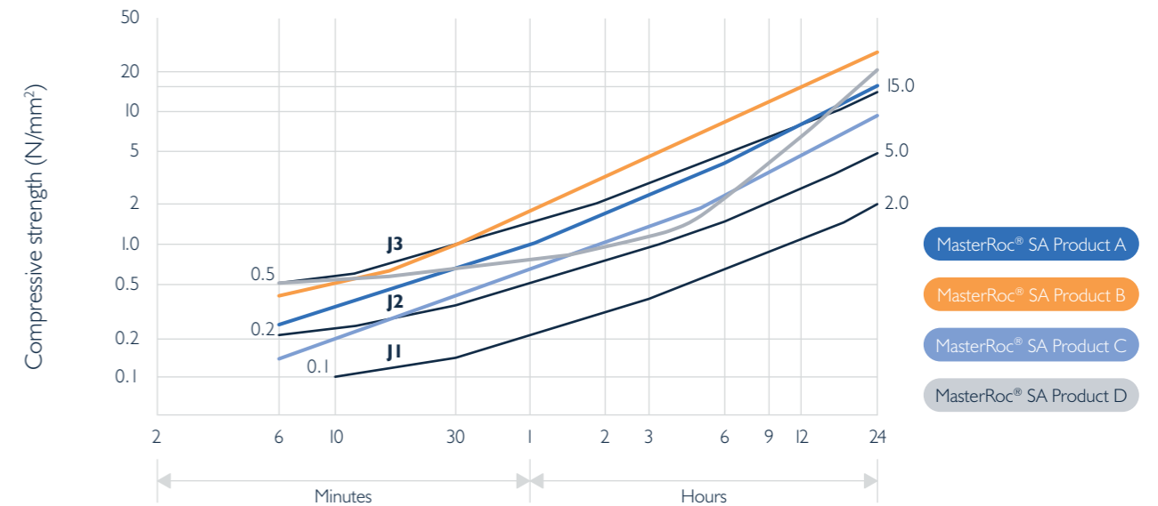
Recorded compressive strength developments by selected alkali-free set accelerators in comparison with J1, J2 and J3 standard requirements based on the Austrian Guideline for sprayed concrete.
