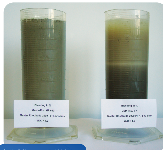
Stable (left) vs. unstable (right) grout
