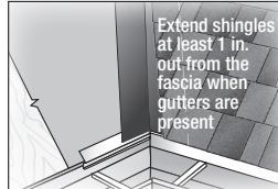
Figure 4.12 Valley/Shingle Extension
