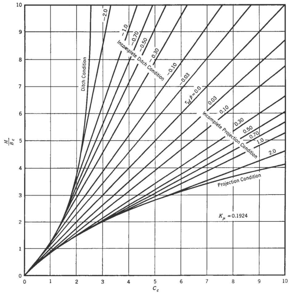
Fig. 1-9. Calculation Coefficients ( C_c ) for Positive-Projection Condition
