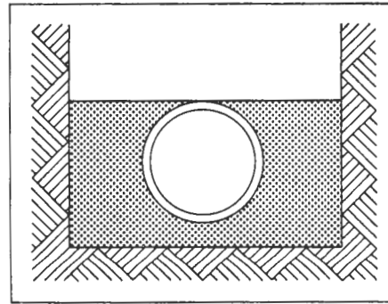
Type 5 Pipe bedded to its centerline in compacted granular material, 4-in. minimum under pipe. Compacted granular or select \frac{1}{2} material to top of pipe. (Approx. 90 per cent Standard Proctor, AASHTO § T-99)
