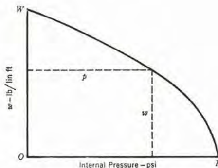
Fig. 1-6. Load-Pressure Curve
