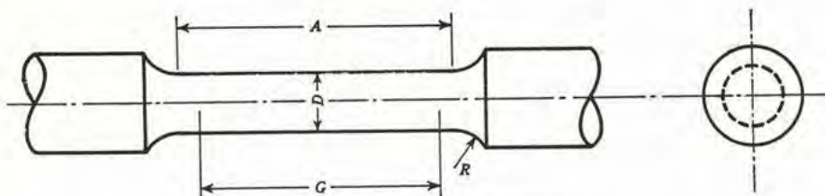
Fig. 1. Tensile-Test Specimen
