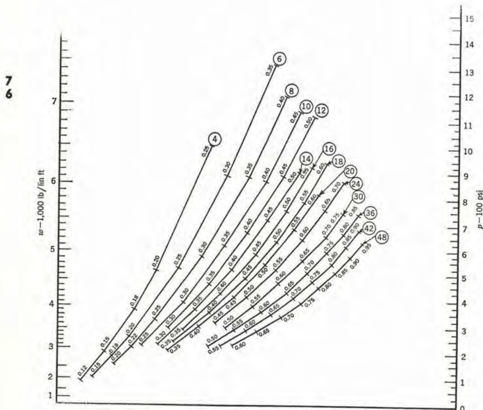
Fig. 1-4. Thickness Nomogram for Pipe of 21/45 Iron Strength, Medium-Range Load Thicknesses are net, and computations are made using nominal pipe diameter for inside diameter. S equals 21,000, R equals 45,000. The encircled values at the end of each curve are for pipe size, in inches.
