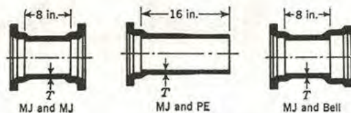
Fig. 10.13. Mechanical-Joint Connecting Pieces (See Table 10.13)
