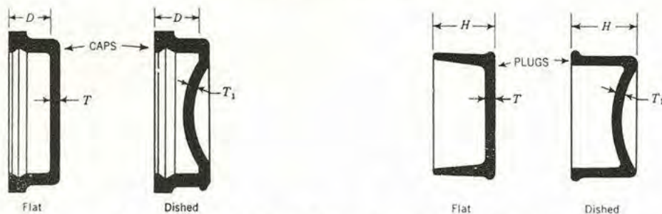
Fig. 10.24. Bell-and-Spigot Caps and Plugs (See Table 10.24)
