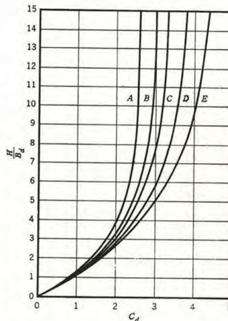
Fig. 1-8. Calculation Coefficients ( C_d ) for Ditch Condition
