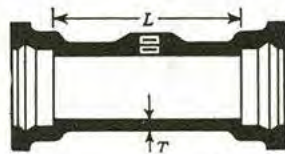
Fig. 10.22. Bell-and-Spigot Tapped Tees (See Table 10.22)
