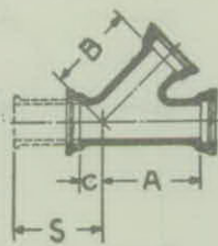
Y-Branch
