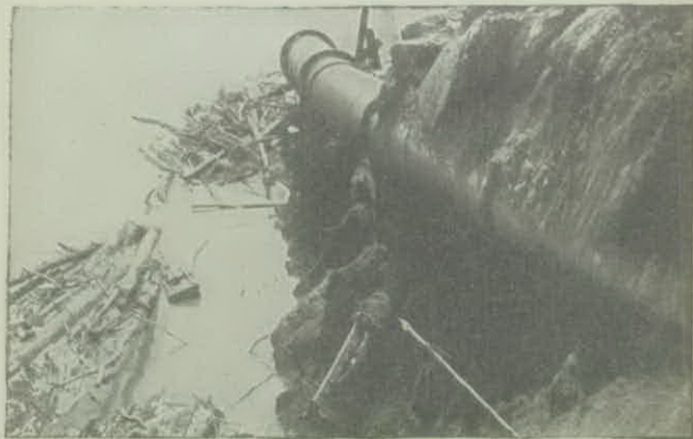
Pipe Line Completely Exposed by Washout of the Supporting Fill
