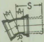
Standard \frac{1}{16} Bend ( 22\frac{1}{2}^\circ )
