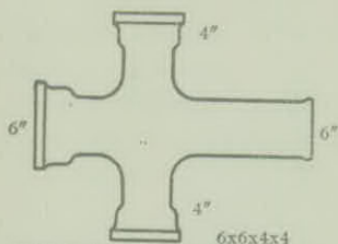
Bell, Spigot, Bell and Bell Cross (B-S-B-B)
