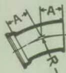
Long Radius \frac{1}{16} Bend ( 22\frac{1}{2}^\circ )
