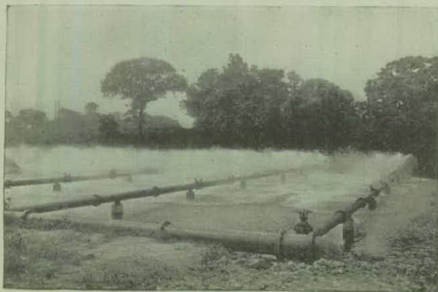
Spray Cooling Pond Piping
