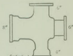
Bell, Flange, Flange and Bell Cross (B-F-F-B)
