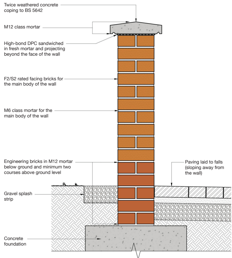
Freestanding Garden Wall Up to 1.2m in height
