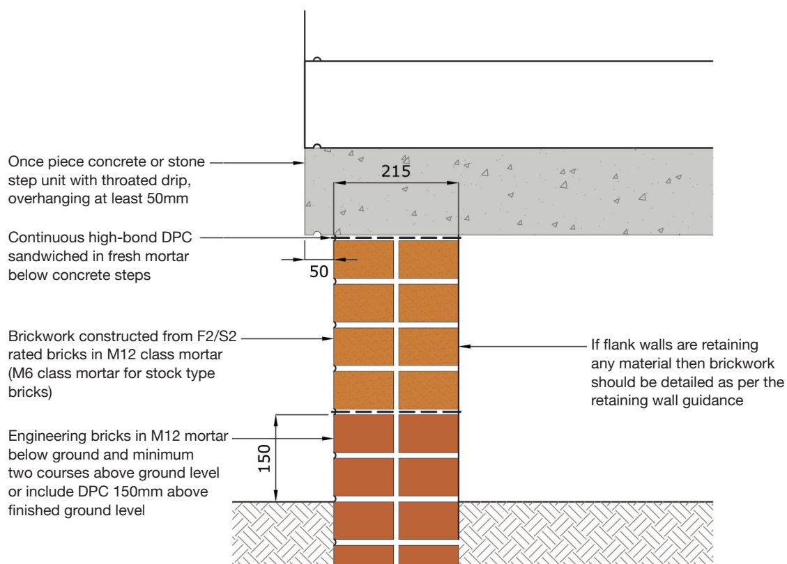
Step Flank Walls Cross Section
