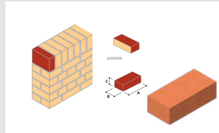
BD.1.3 Standard Brick fair-faced On Bed Surface
