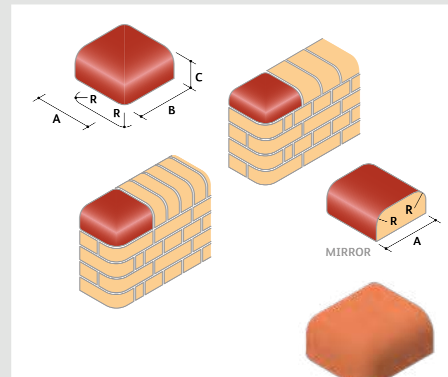
BN.18 Stop End to Double Bullnose On Edge and to Bullnose Double Header On Flat (Rounded Corners On Bed)
