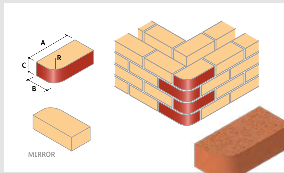
BN.1 Single Bullnose (Left & Right Hand)
