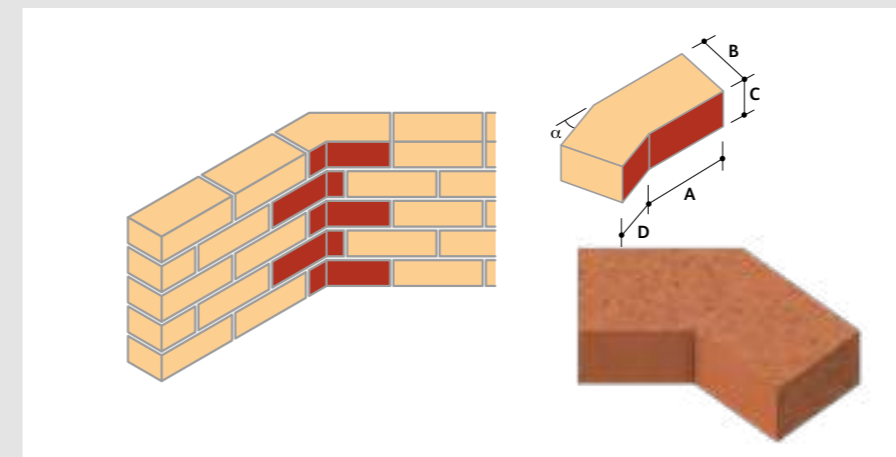
AN.3 Internal Angle (Dog Leg) (Left & Right Hand)
