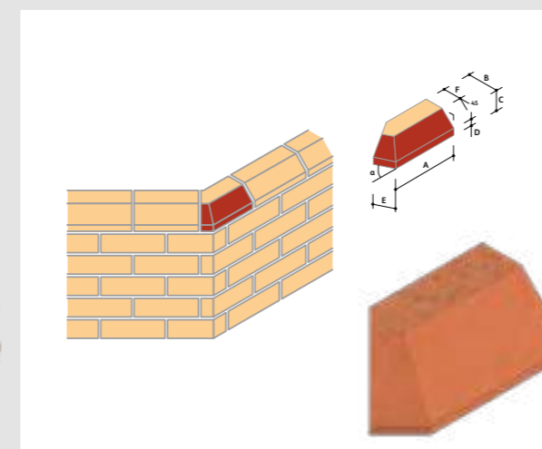
PL.9 Plinth Squint (Left & Right Hand)*
