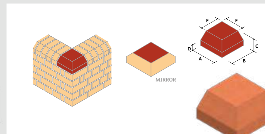
AN.7 Single Cant External Return ⓘ
