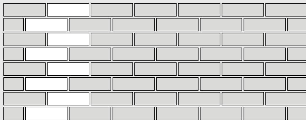
Stretcher bond
