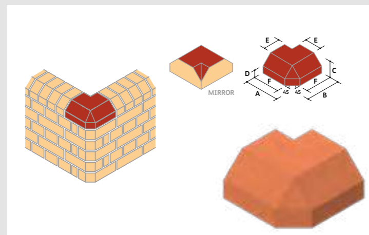
AN.15 Double Cant External Return with Internal Mitre (Canted Corner On Bed)
