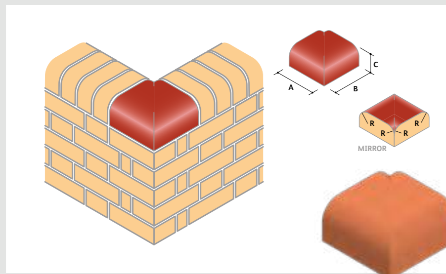
BN.19 External Return to Double Bullnose On Edge and to Bullnose Double Header On Flat (Square Corner On Bed)
