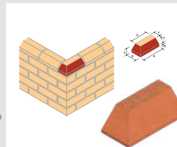
PL.7 Plinth Internal Return - short (Left & Right Hand)*
