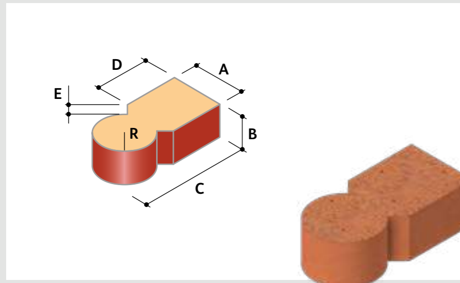
I.U.J.1 Universal Joint Male
