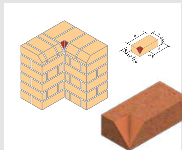
PL.5 Plinth Internal Return - short (Left & Right Hand)*
