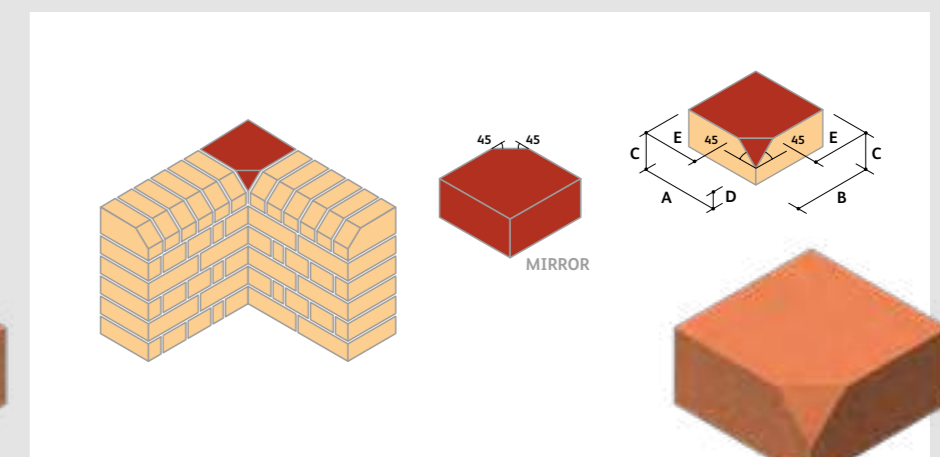
AN.9 Single Cant Internal Return w/ Int. Slope (Sq. External Corner On Bed) ⓘ
