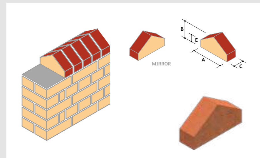
CP.2.2 Saddleback Capping ⓘ
