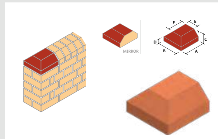
AN.12 Double Cant Stop End (Square Corners On Bed)
