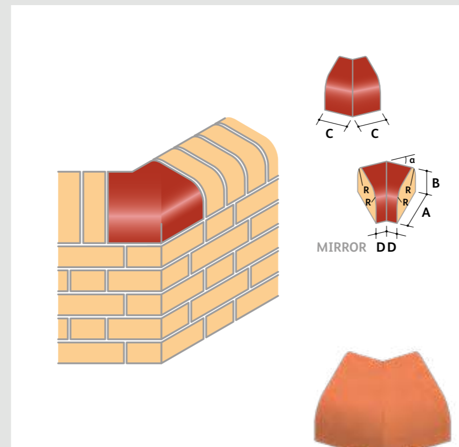
BN.21 Double Bullnose External Angle to Double Bullnose On Edge and to Bullnose Double Header On Flat
