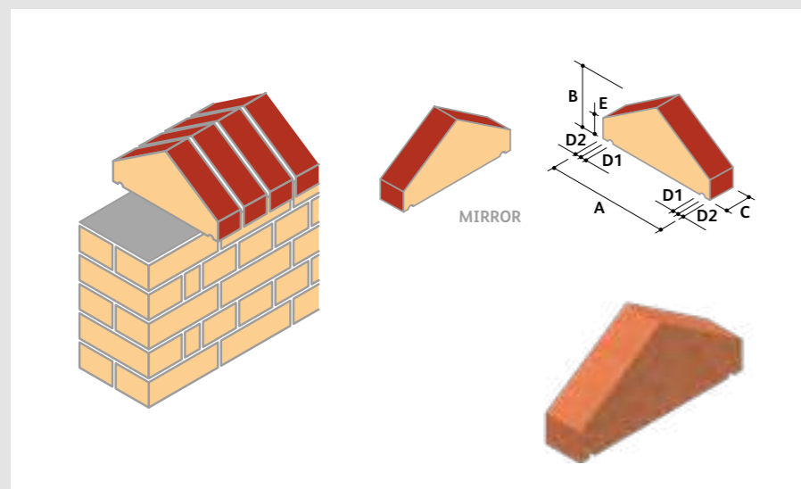
CP.2.1 Saddleback Copping ⓘ
