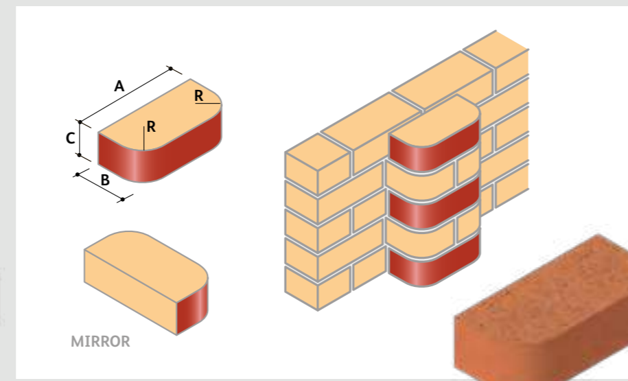
BN.2 Double Bullnose
