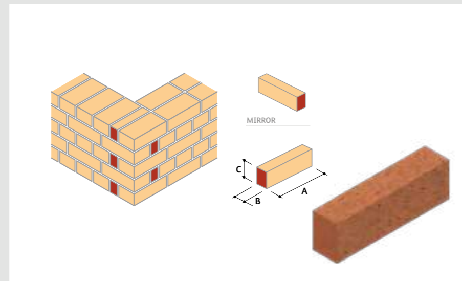
BD.3 Queen Closer
