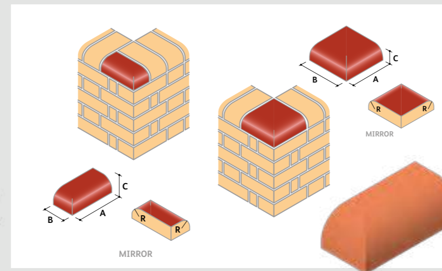
BN.11 Bullnose External Return On Flat (Left & Right Hand)
