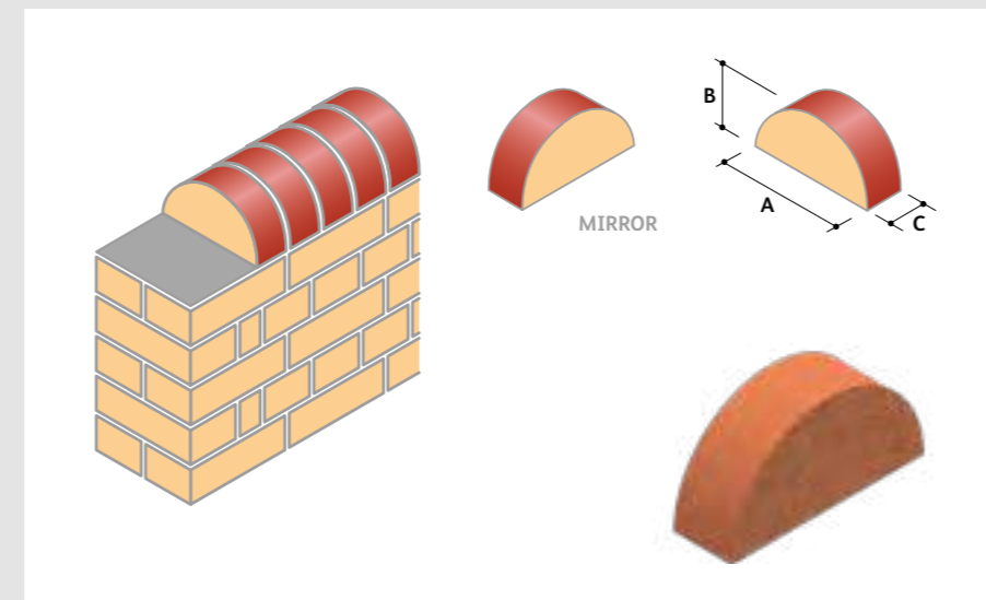
CP.1.2 Half Round Capping ⓘ
