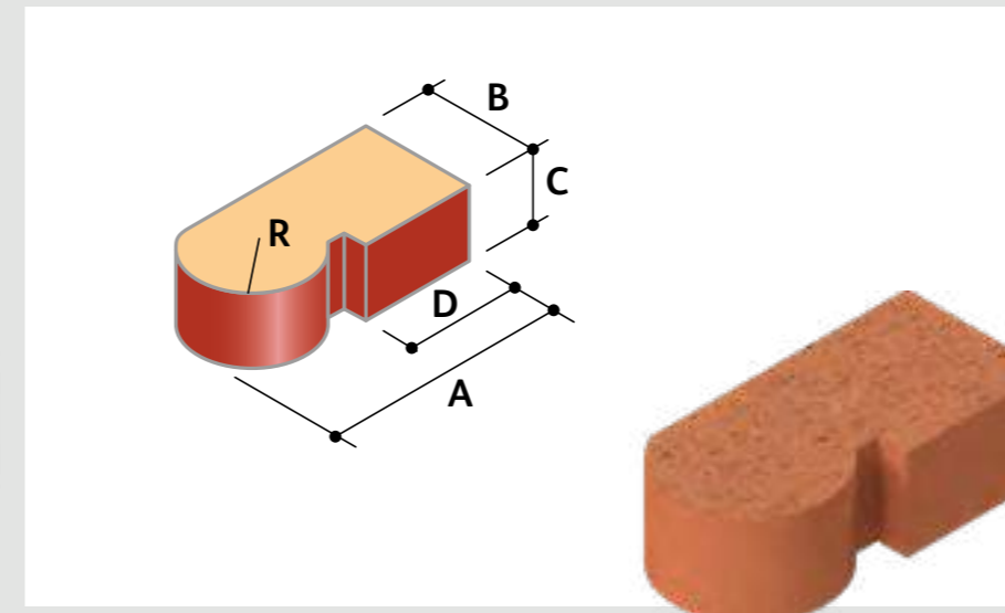
I.U.J.7 Easyangle® (Left & Right Hand)
