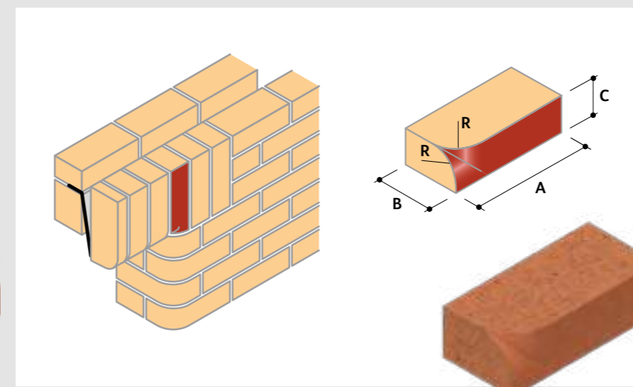
BN.7 Single Bullnose Internal Return Stretcher Faced (Left & Right Hand)
