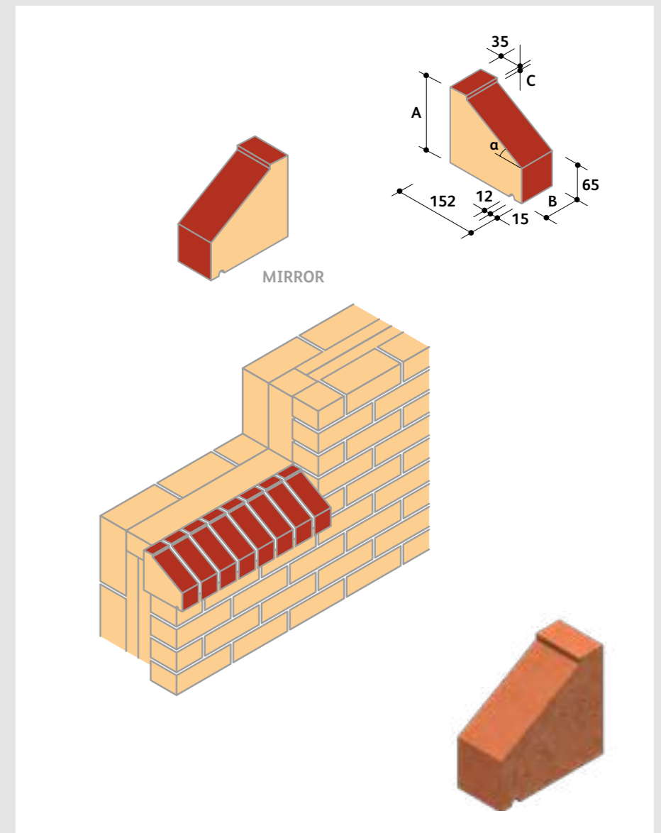
I.C.1 Overhanging Angled Sill
