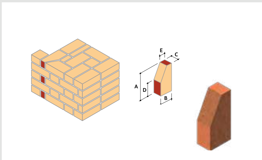
BD.2 King Closer
