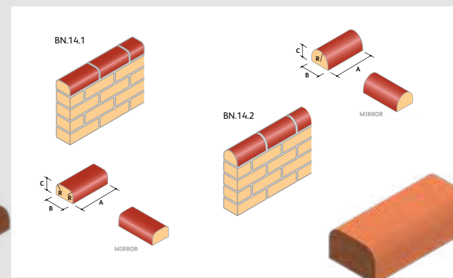
BN.14 Bullnose Double Stretcher On Flat
