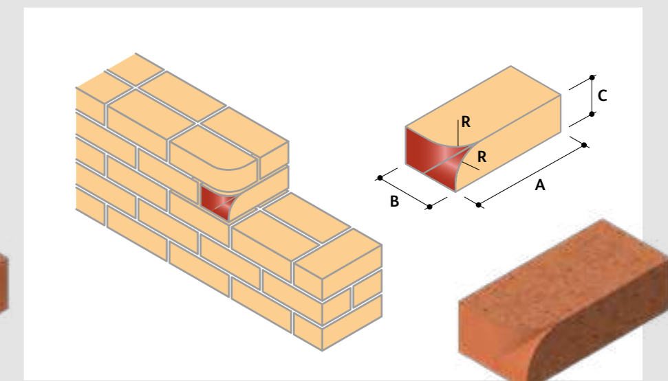
BN.8 Single Bullnose Internal Return Header Faced (Left & Right Hand)
