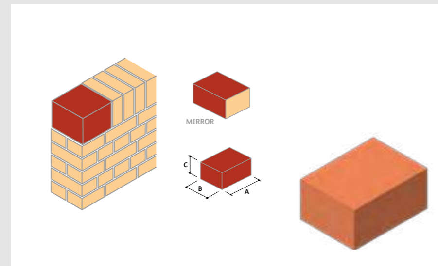
BD.4 215mm Square Stop End
