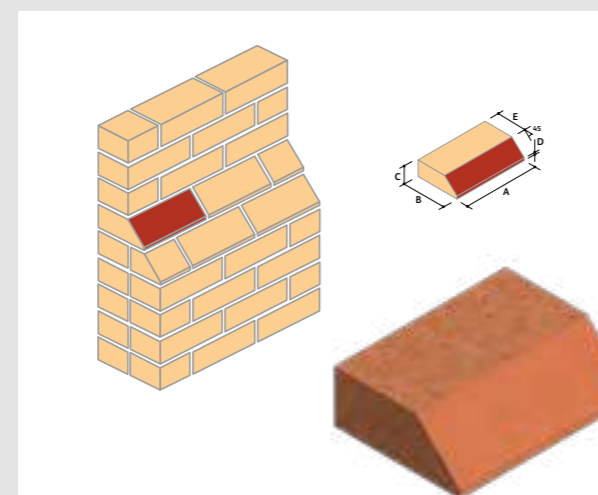
I.PL.15 Wide Bed Plinth Stretcher
