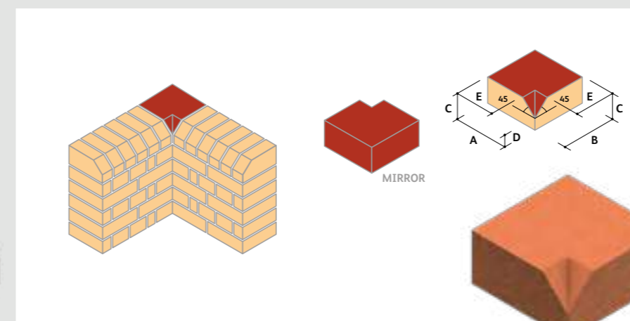
AN.8 Single Cant Internal Return w/ Int. Mitre (Sq. External Corner On Bed) ⓘ
