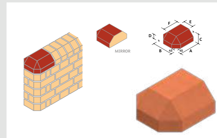
AN.13 Double Cant Stop End (Canted Corners On Bed)
