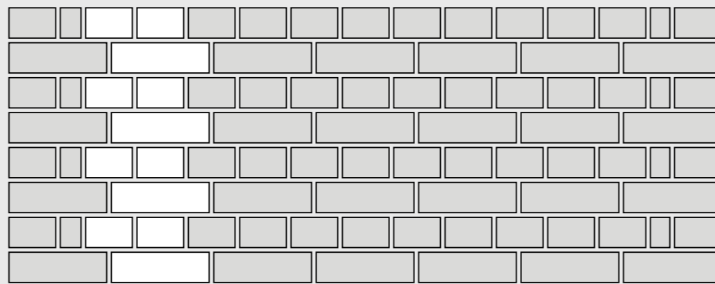
English bond
