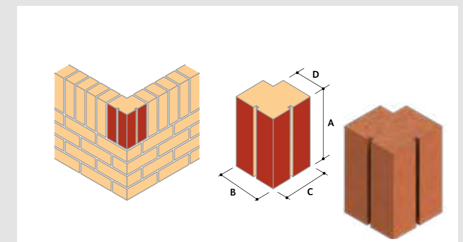
I.SD.4 Soldier External Return
