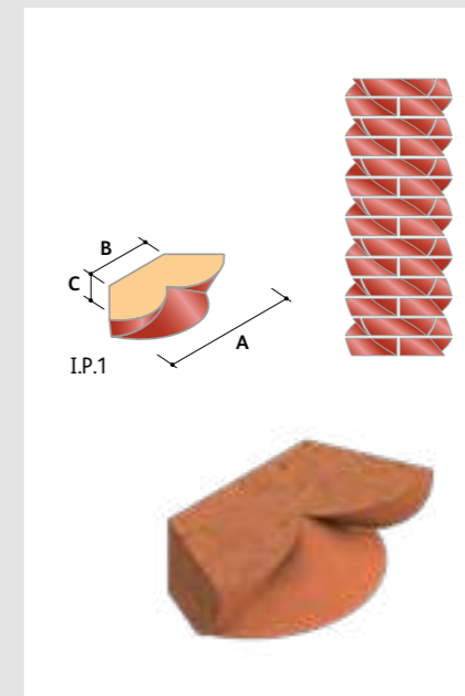
I.P.1 Pineapple Brick To 400mm Diameter Column
