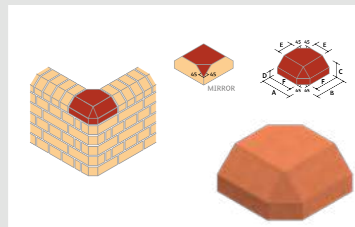
AN.17 Double Cant External Return with Internal Slope (Canted Corners On Bed)
