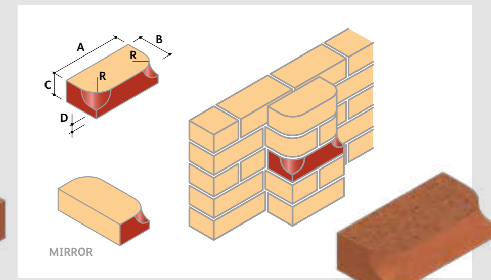
BN.4 Double Bullnose Stop
