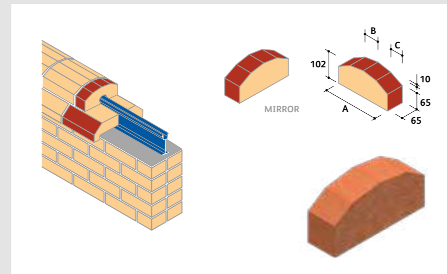
I.F.1 Faceted Copping + ⓘ
