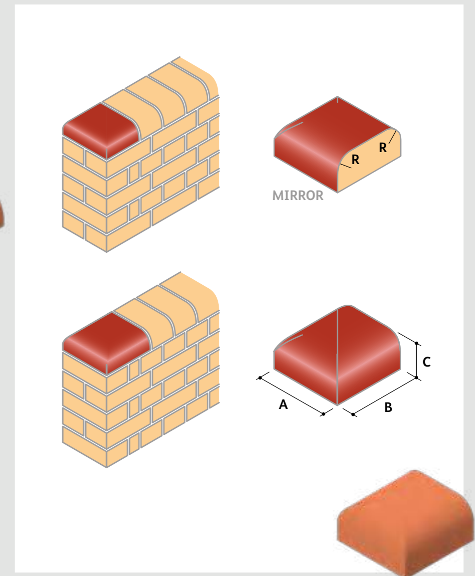
BN.15 Stop End to Double Bullnose On Edge and to Bullnose Double Header On Flat (Square Corners On Bed)
