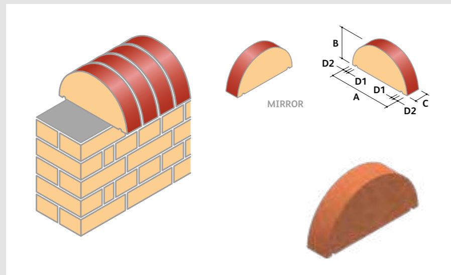
CP.1.1 Half Round Copping ⓘ
