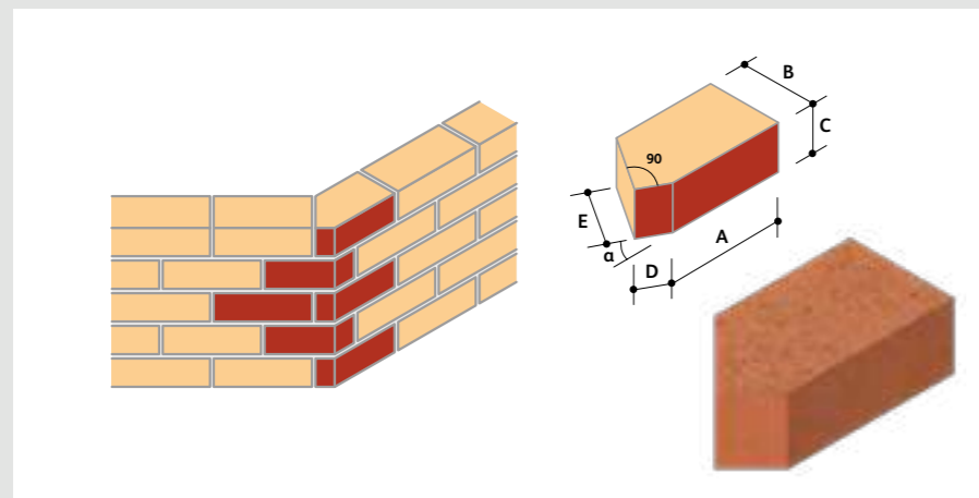
AN.1 Squint Brick (Left & Right Hand)
