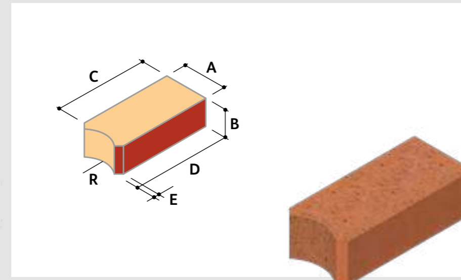
I.U.J.2 Universal Joint Female
