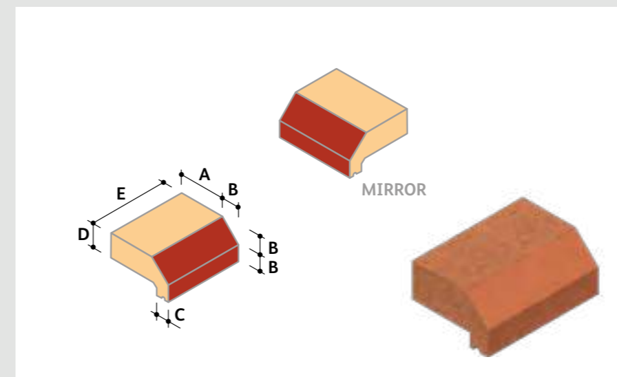
I.B.C.1 Base Copping Standard Brick**
