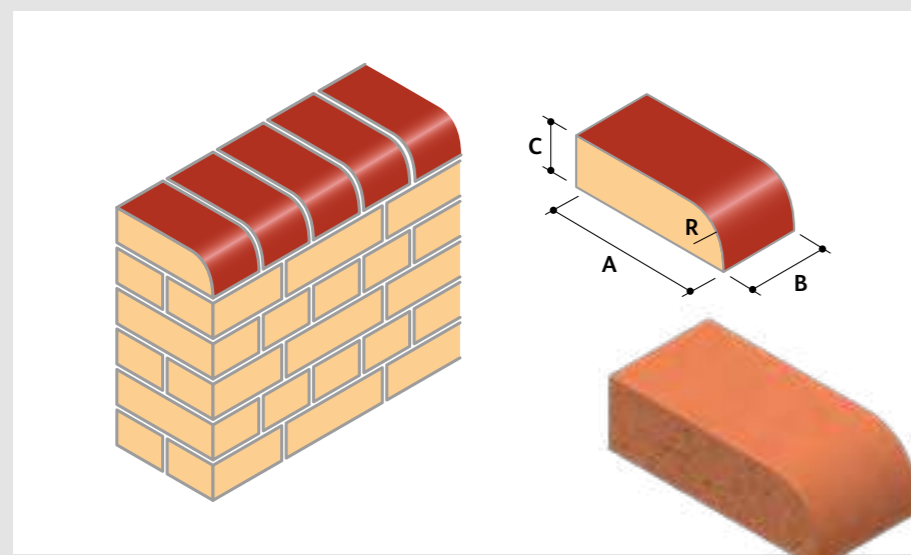
BN.5 Single Bullnose Header On Flat
