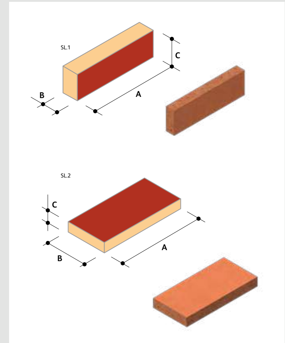
SL.1 Brick Face Slip
