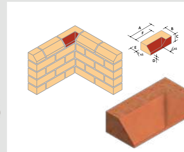
PL.4 Plinth Internal Return - long (Left & Right Hand)*
