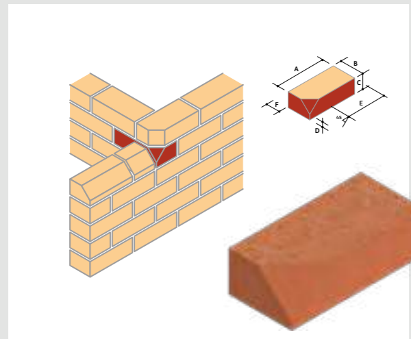
PL.1 Plinth Stop Or Cant Stop (Left & Right Hand)*
