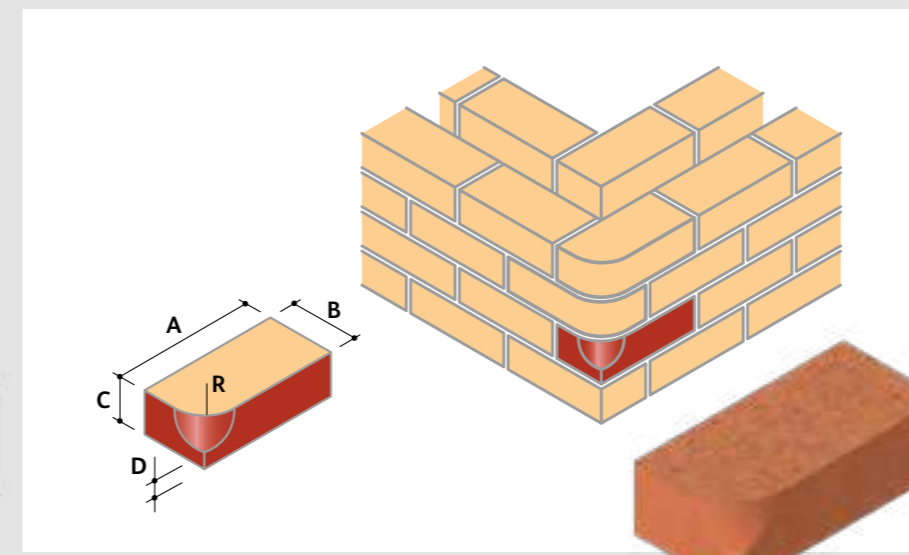
BN.3 Single Bullnose Stop (Left & Right Hand)
