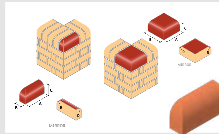
BN.10 Bullnose External Return On Edge (Left & Right Hand)
