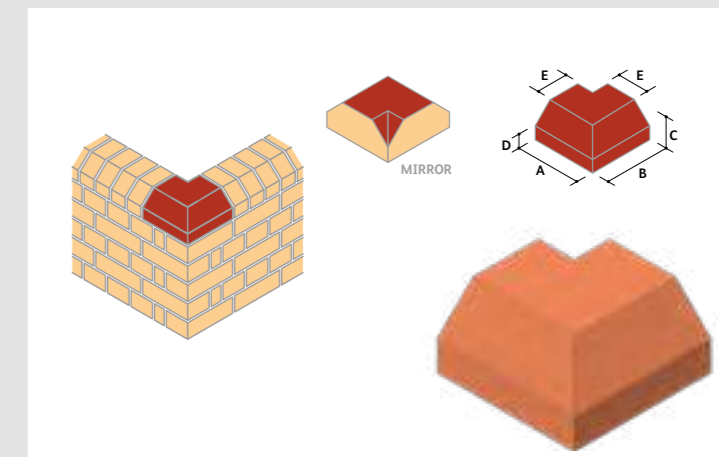
AN.14 Double Cant External Return with Internal Mitre (Square Corner On Bed)
