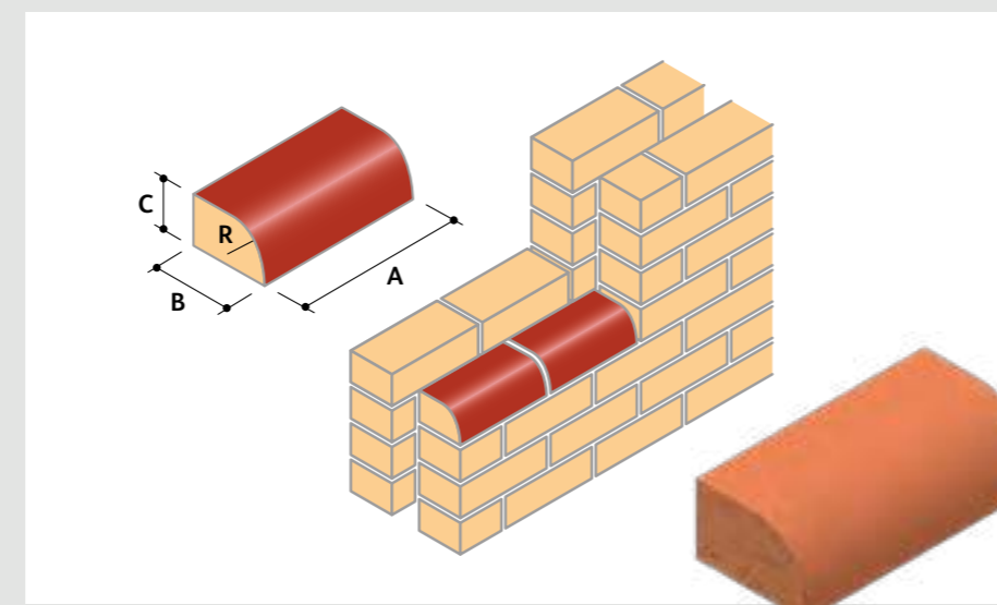
BN.6 Single Bullnose Stretcher On Flat
