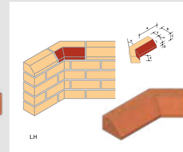
PL.6 Plinth Internal Angle (Left & Right Hand)*
