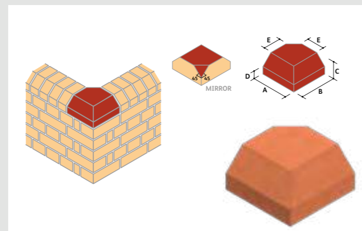
AN.16 Double Cant External Return with Internal Slope (Square Corner On Bed)
