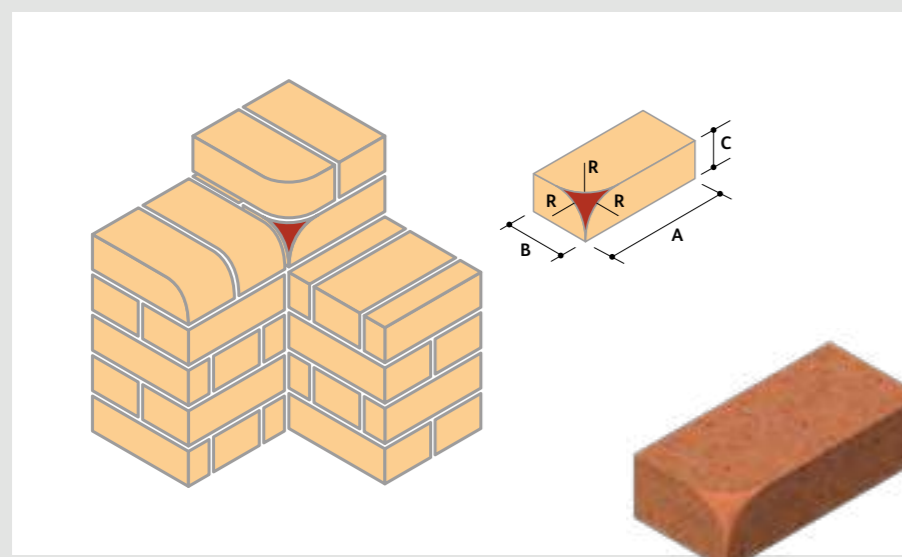
BN.12 Bullnose Mitre (Left & Right Hand)
