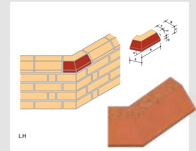
PL.8 Plinth External Angle (Left & Right Hand)*
