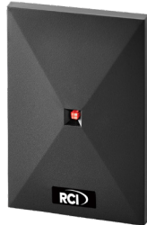
P-500-H-A 125kHz Reader Compact design ideal for single gang wall-box applications. 3"W x 4-5/8"H x 3/8"D (76 x 117 x 10mm)
