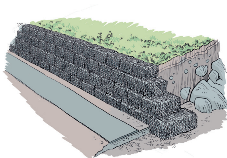
Skiss gravitationsmur
