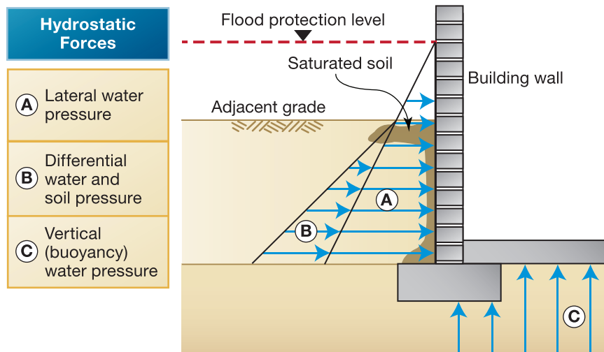
Figure 1-4. Hydrostatic forces.
