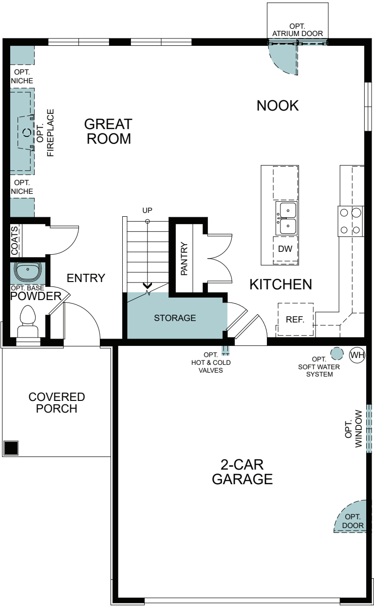
FIRST FLOOR 750 SQ. FT.
