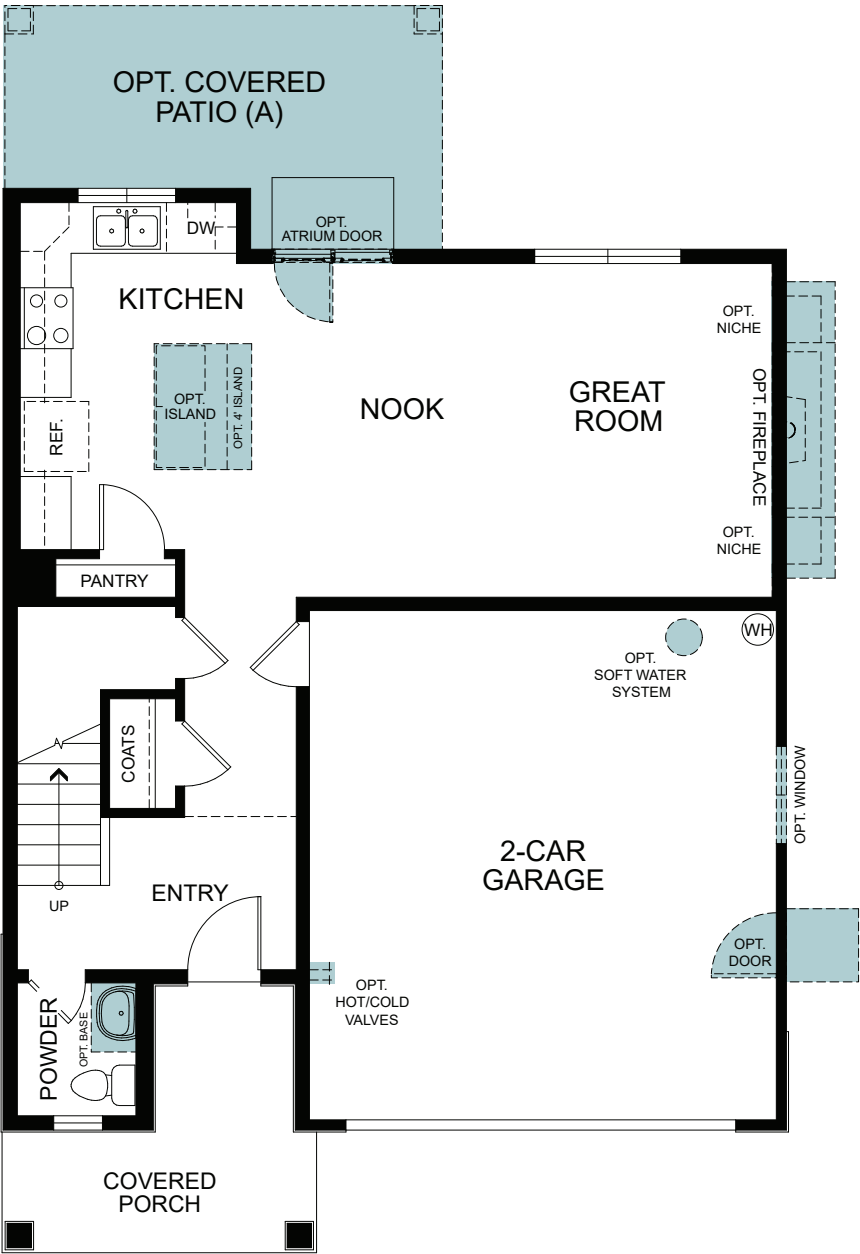
FIRST FLOOR 708 SQ. FT.
