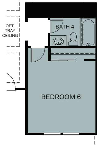
OPTIONAL BEDROOM 6 AND BATH 4 ILO FLEX SPACE
