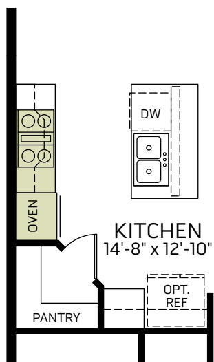
OPTIONAL KITCHEN APPLIANCE LAYOUT
