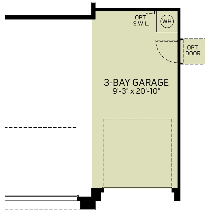
OPTIONAL 3-BAY GARAGE (LENGTH OF 3-BAY GARAGE DOES NOT EXTEND WITH 2 FT. AND 4 FT. GARAGE EXTENSIONS.)
