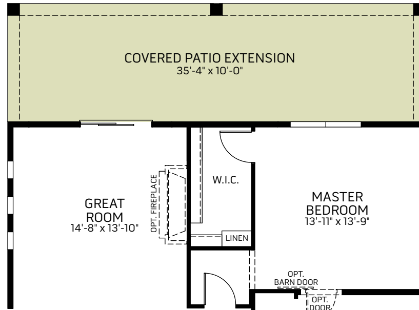
OPTIONAL COVERED PATIO EXTENSION
