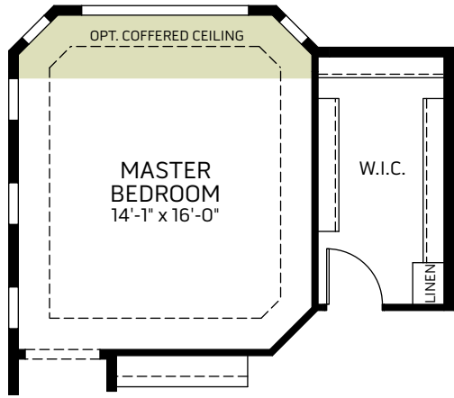
OPTIONAL BAY WINDOW AT MASTER BEDROOM (NOT AVAILABLE WITH MASTER BEDROOM EXTENSION OR WORK FROM HOME OPTIONS)
