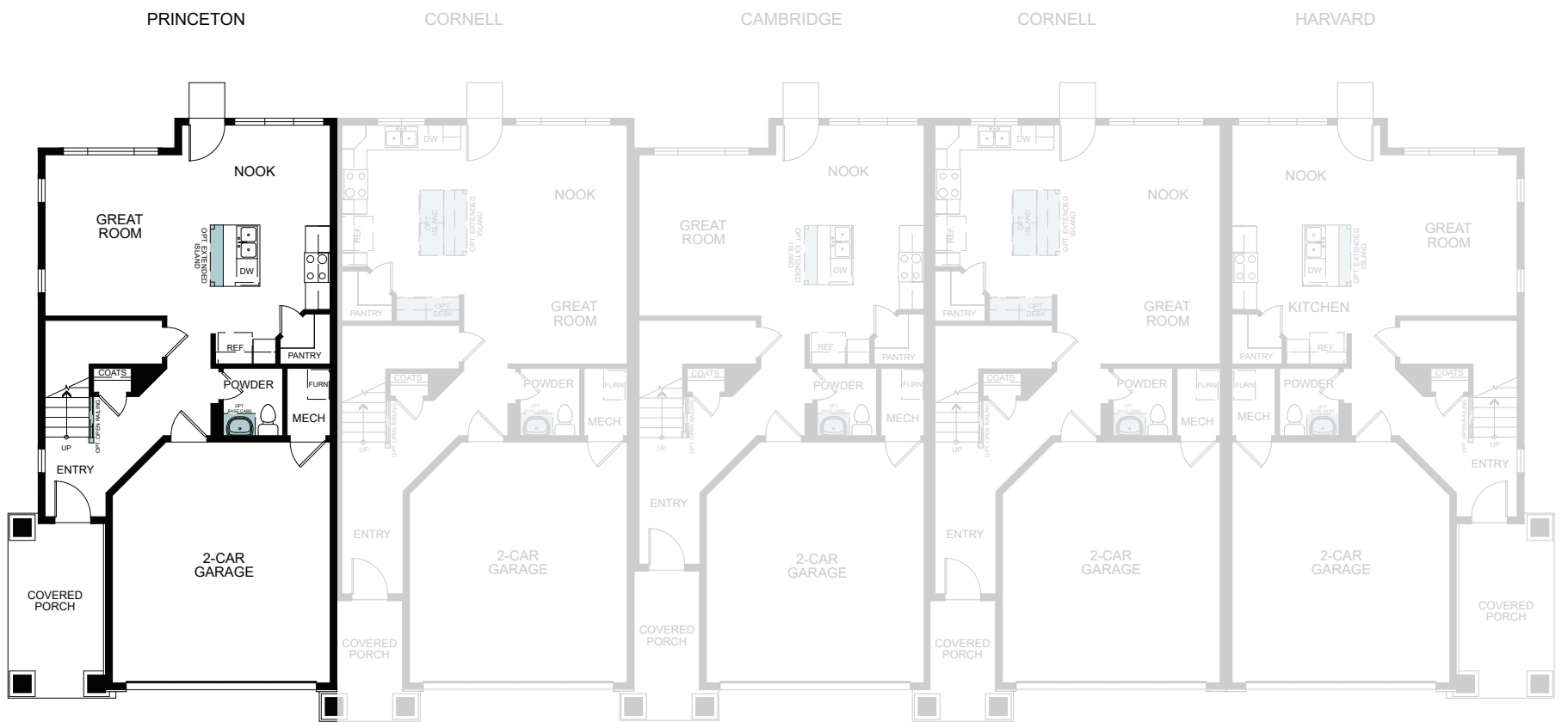
FIRST FLOOR 692 Sq. Ft.
