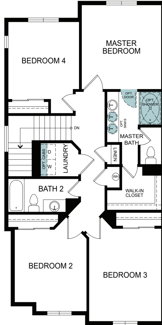
SECOND FLOOR 1,078 Sq. Ft.
