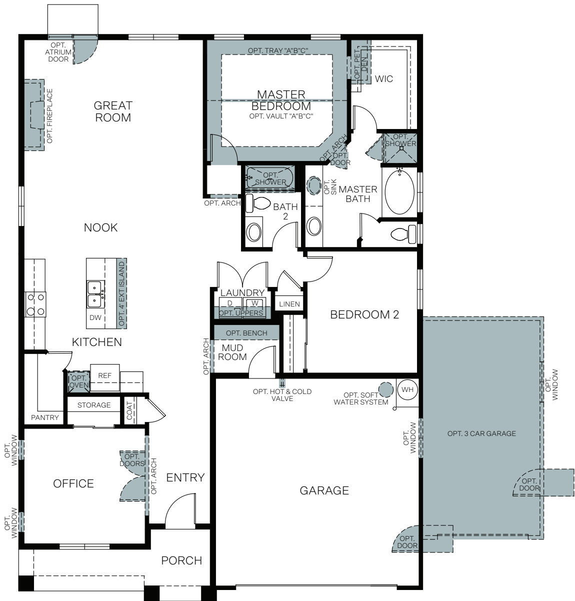
FIRST FLOOR 1,616 Sq.Ft.
