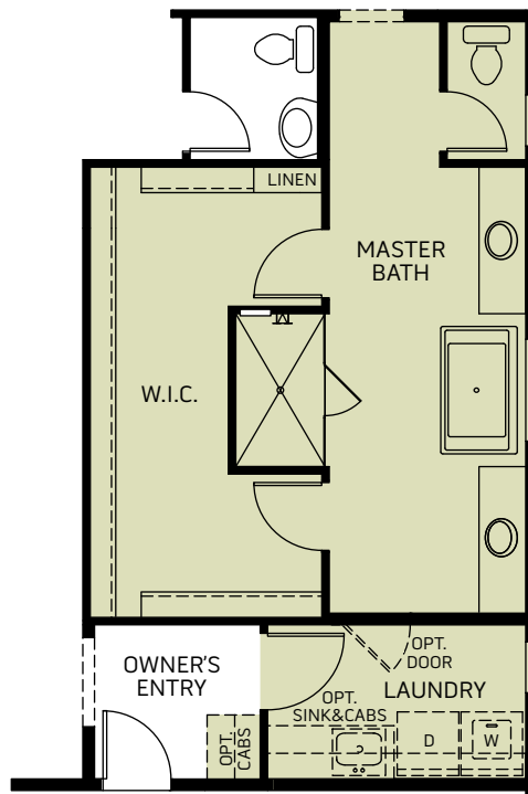
OPTIONAL LUXURY MASTER BATHROOM (NOT AVAILABLE WITH BONUS ROOM) (NOT AVAILABLE WITH SUPER LAUNDRY OPTIONS)
