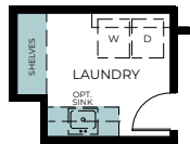
OPTIONAL SINK AND CABINETS
