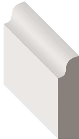
STOCK CODE 905LP (1522275) DIMENSIONS \frac{7}{16}'' \times 1\frac{5}{8}'' \times 16' PFJ
