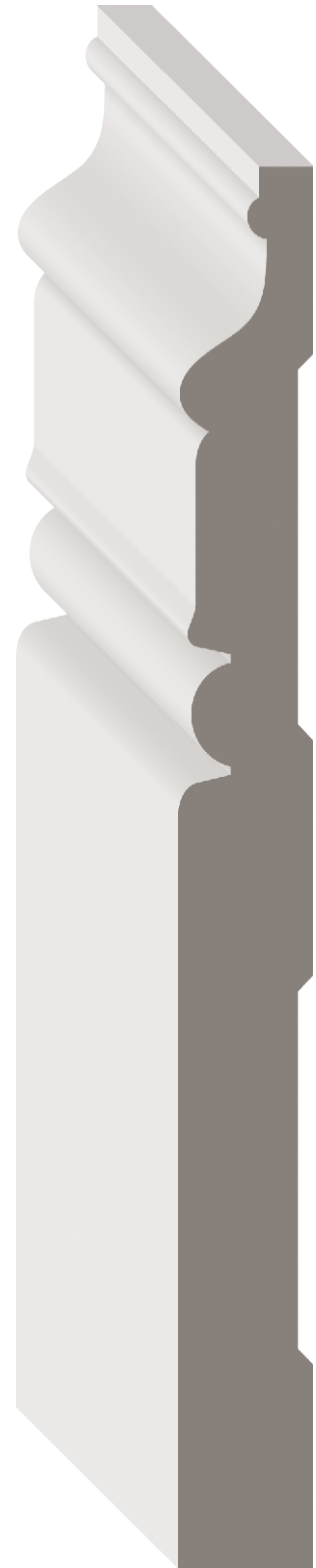
STOCK CODE 20232EBM (1484570) DIMENSIONS 5/8" x 7 1/4" x 16' MDF/UL
