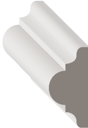
STOCK CODE 2448BMFJP (1521624) DIMENSIONS \frac{3}{4} " x 1\frac{1}{2} " x 16' RFJ
