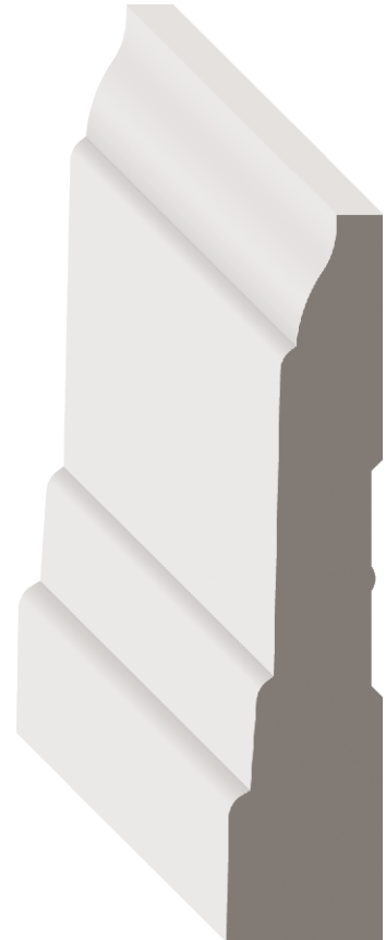
STOCK CODE 9832PRI (1522380) DIMENSIONS \frac{3}{4}'' \times 3\frac{1}{2}'' \times 16' PRI
