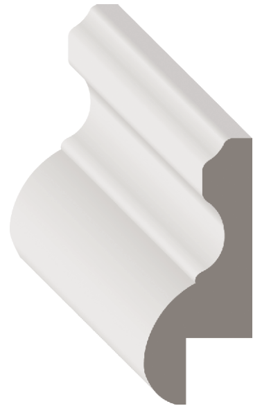
STOCK CODE 2664PRPOP (1521694) DIMENSIONS 1\frac{3}{16}'' \times 2'' \times \text{RL} \frac{1}{2}'' \times 1\frac{1}{2}'' RABBET POP
