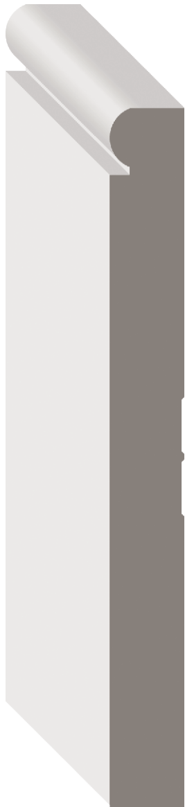
STOCK CODE 1382988 DIMENSIONS \frac{1}{2} " x 5\frac{1}{4} " x 16' MDF/UL
