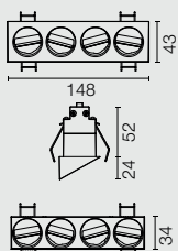
POWER LED 2,7W x SPOT
