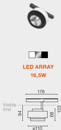
ANTHONY SPOT TRACK
