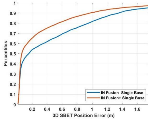
Figure 9: AP+ 30 SBET Position Errors CDF
