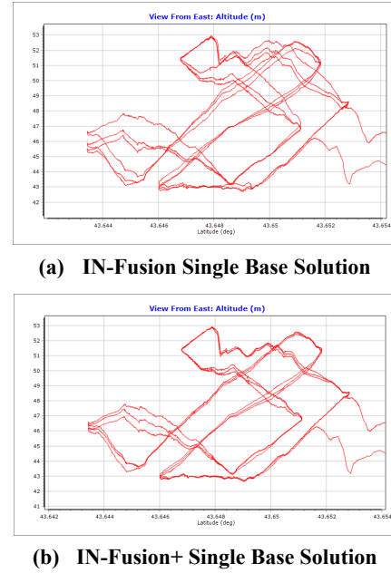
Figure 5: Altitude vs Latitude SBET Trajectories in Dense Urban Areas
