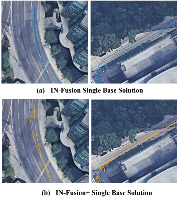
Figure 4: Horizontal SBET Trajectories in Dense Urban Areas
