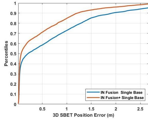
Figure 8: LVX SBET Position Errors CDF
