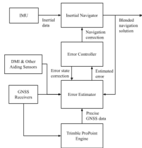
Figure 3: Trimble® Applanix IN-Fusion+™ Architecture
