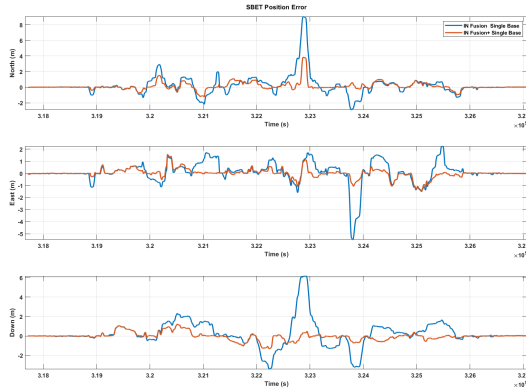
Figure 7: SBET Position Errors for One Dataset
