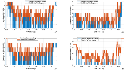
Figure 1: Number of Satellites Used
