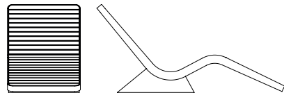
FRV0002 Lounger 1,675 x 660 mm • H 800 mm
