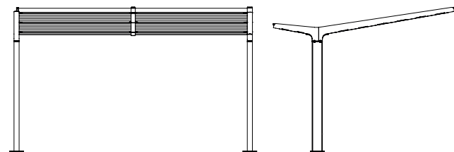
SUT1000 Shade SUT1001 Shade with wood cladding 5.11 × 3.92 m • H 3.10 m Capacity: 2 cars SUT1002 PRM Shade 3.42 × 3.92 m • H 3.10 m Capacity: 1 car
