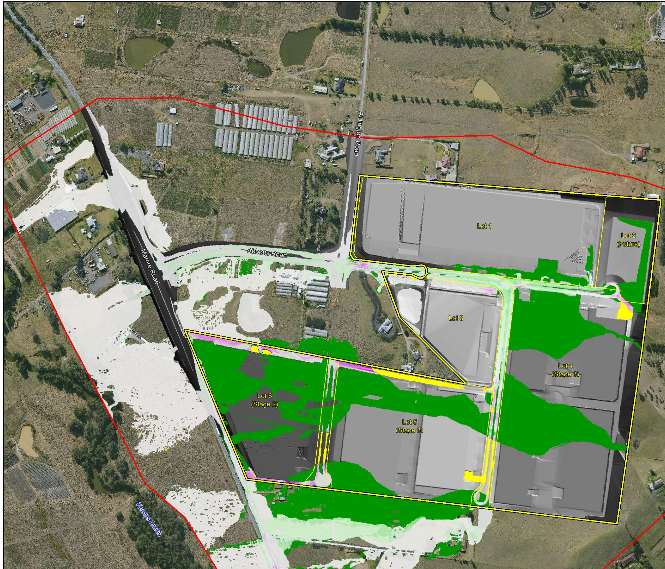
Figure 5-28 Westlink Stage 2, Lot 4 & Lot 5 Flood Impact and Risk 0.5% AEP Developed minus Base Conditions Flood Velocity Difference
