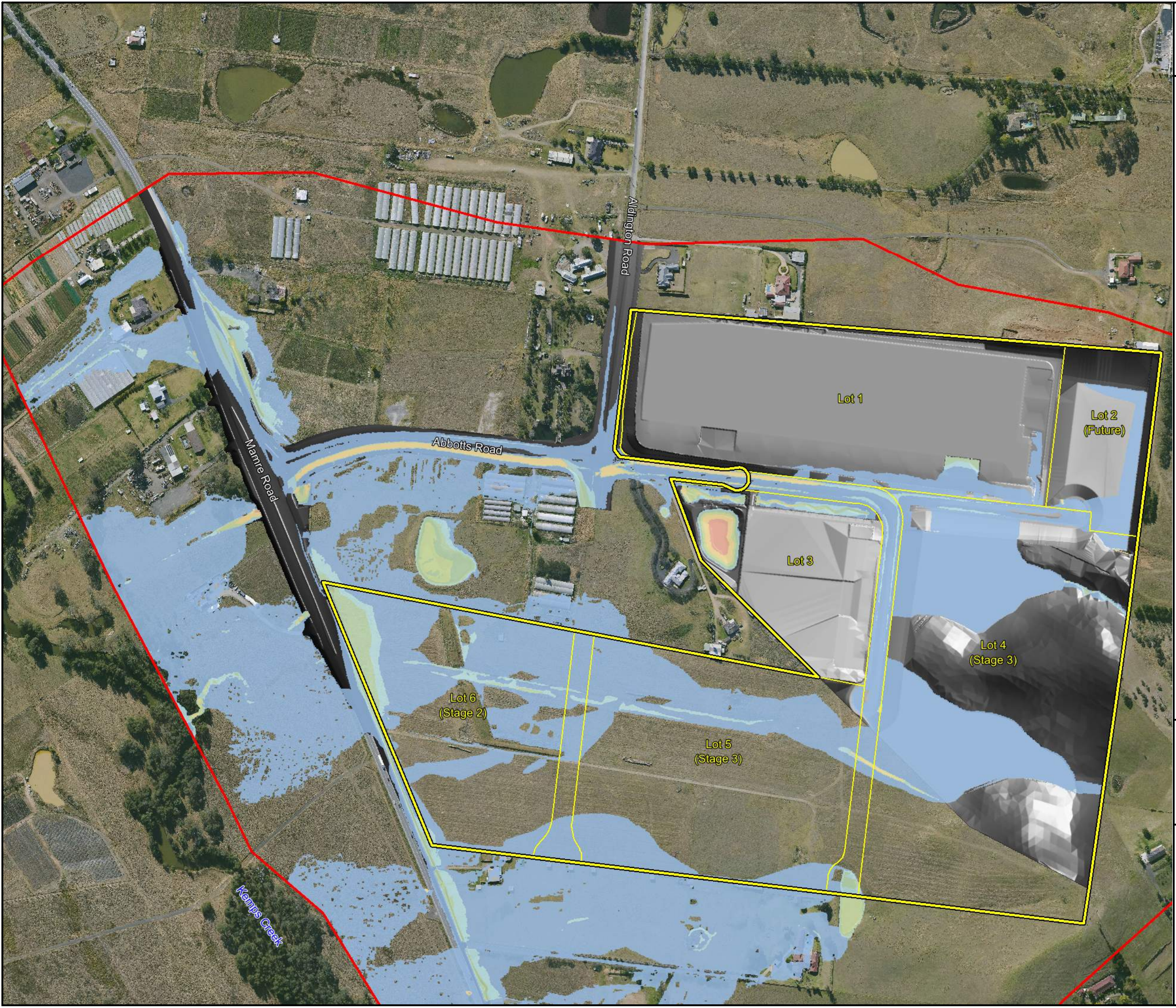
Figure 5-33 Westlink Stage 2, Lot 4 & Lot 5 Flood Impact and Risk 0.5% AEP Base Conditions NoTW Flood Hazard
