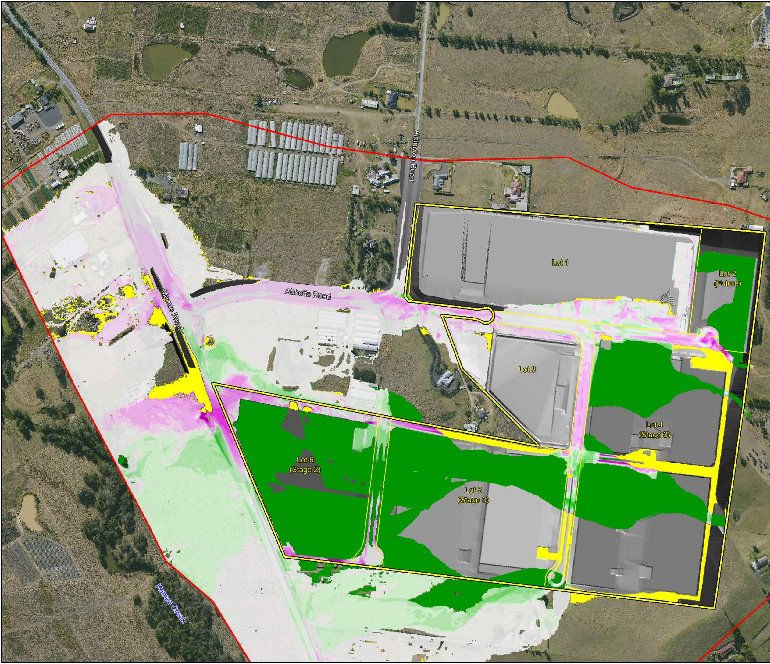
Figure 5-30 Westlink Stage 2, Lot 4 & Lot 5 Flood Impact and Risk PMF Developed minus Base Conditions Flood Velocity Difference
