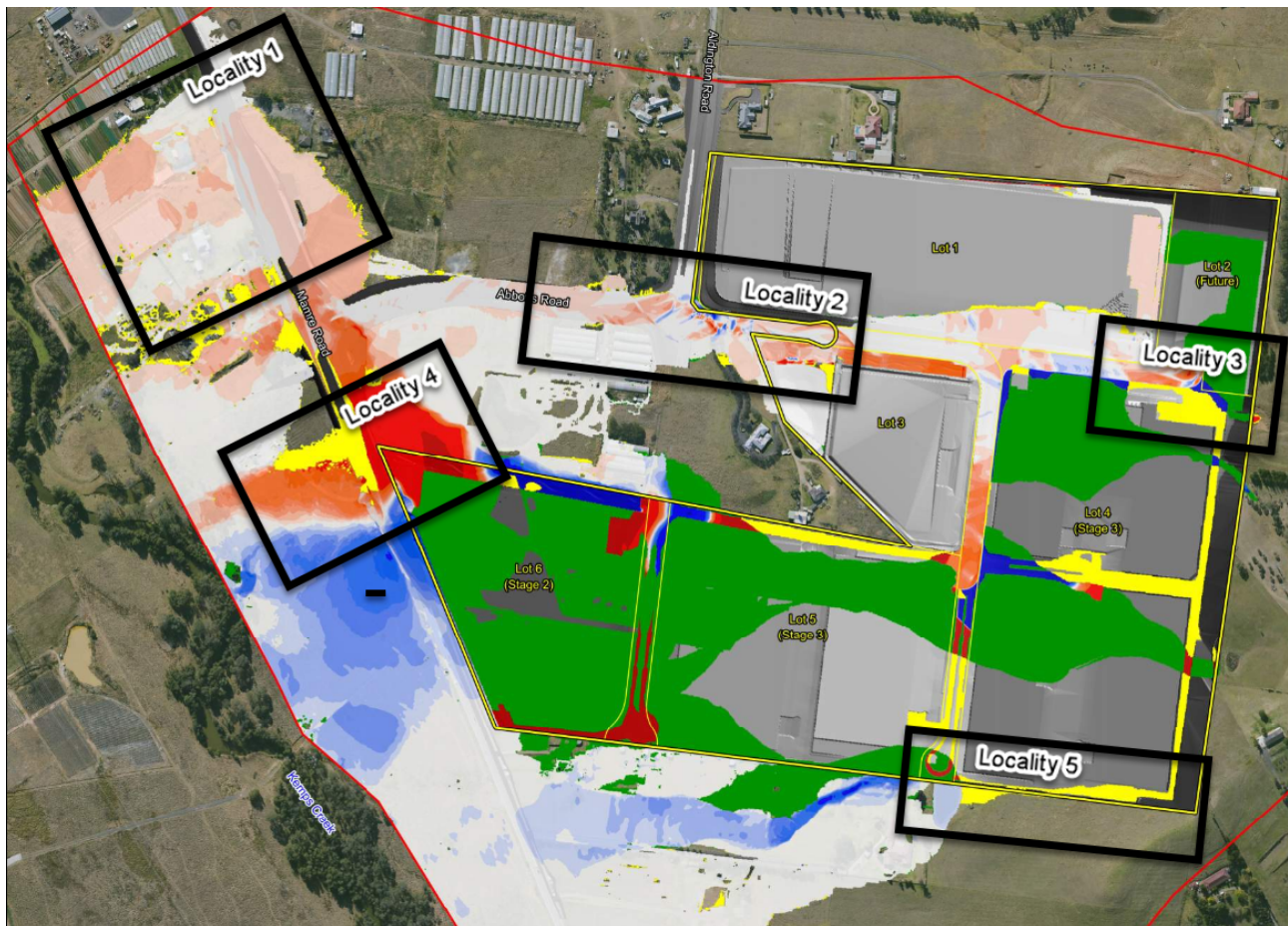
Plate 5-3 – Locality/Inset Key Map overlaid on PMF Flood Level Difference Map
