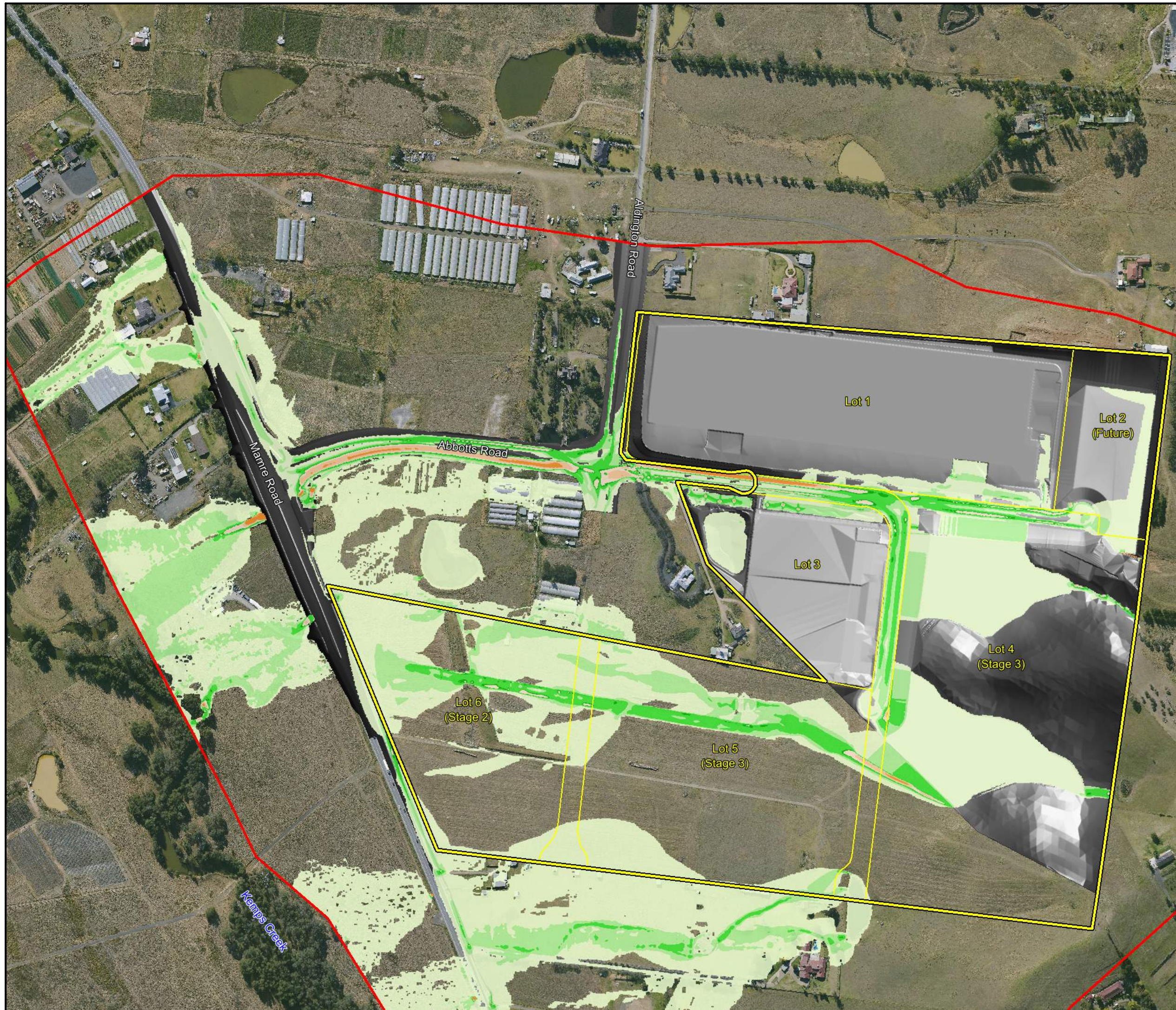
Figure 5-17 Westlink Stage 2, Lot 4 & Lot 5 Flood Impact and Risk 1% AEP Base Conditions NoTW Flood Velocity
