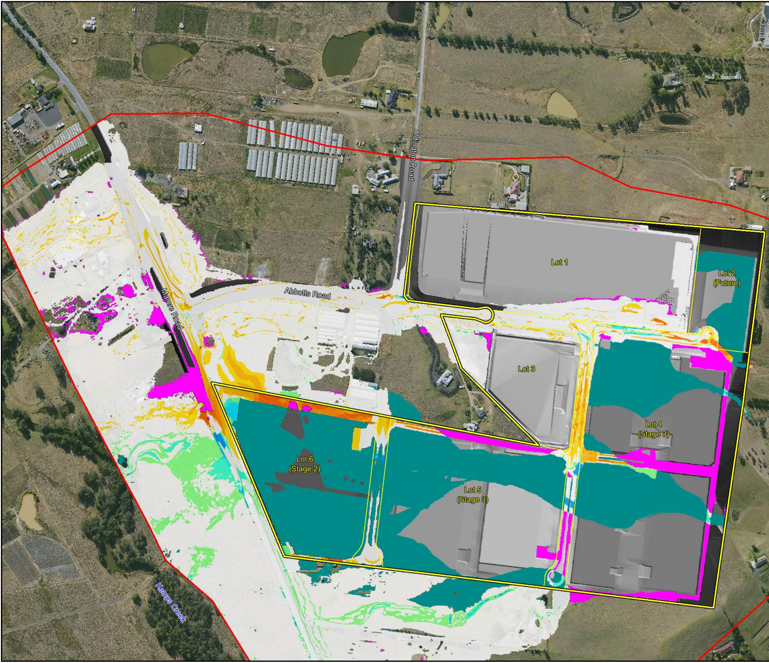
Figure 5-45 Westlink Stage 2, Lot 4 & Lot 5 Flood Impact and Risk PMF Developed minus Base Conditions Flood Hazard Difference
