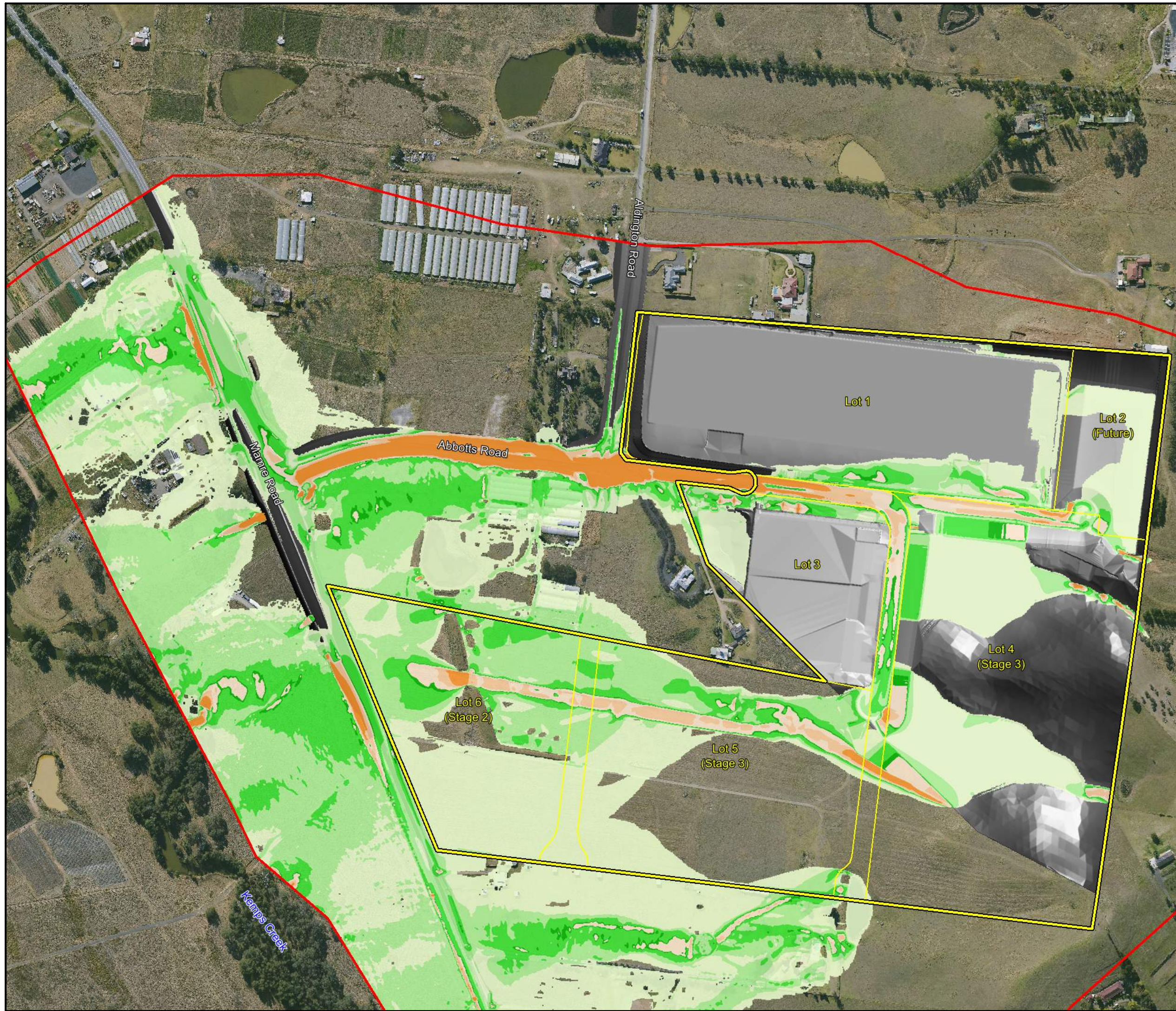
Figure 5-20 Westlink Stage 2, Lot 4 & Lot 5 Flood Impact and Risk PMF Base Conditions NoTW Flood Velocity
