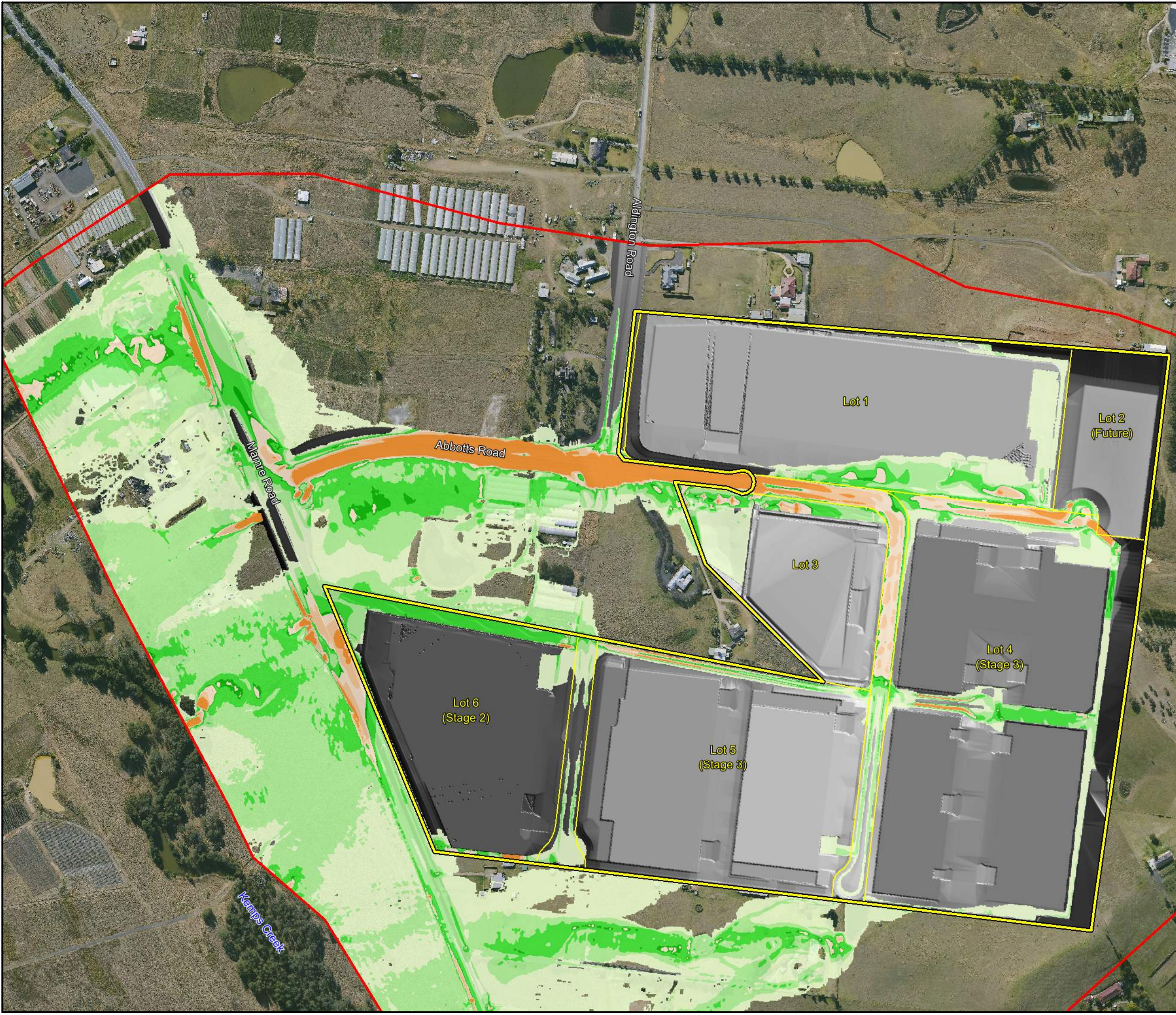
Figure 5-25 Westlink Stage 2, Lot 4 & Lot 5 Flood Impact and Risk PMF Developed Conditions NoTW Flood Velocity
