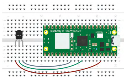
■ The TMP36 temperature sensor connected to Raspberry Pi Pico
