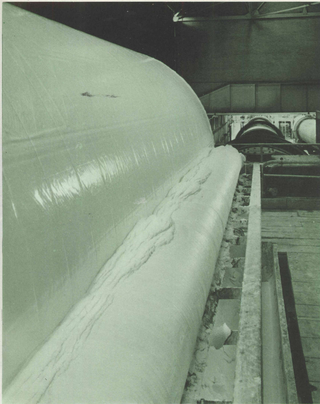
White titanium pigment production ; the pigment is scraped off the roller and then passed by conveyor belt to the dryers. Laporte Industries Ltd.
