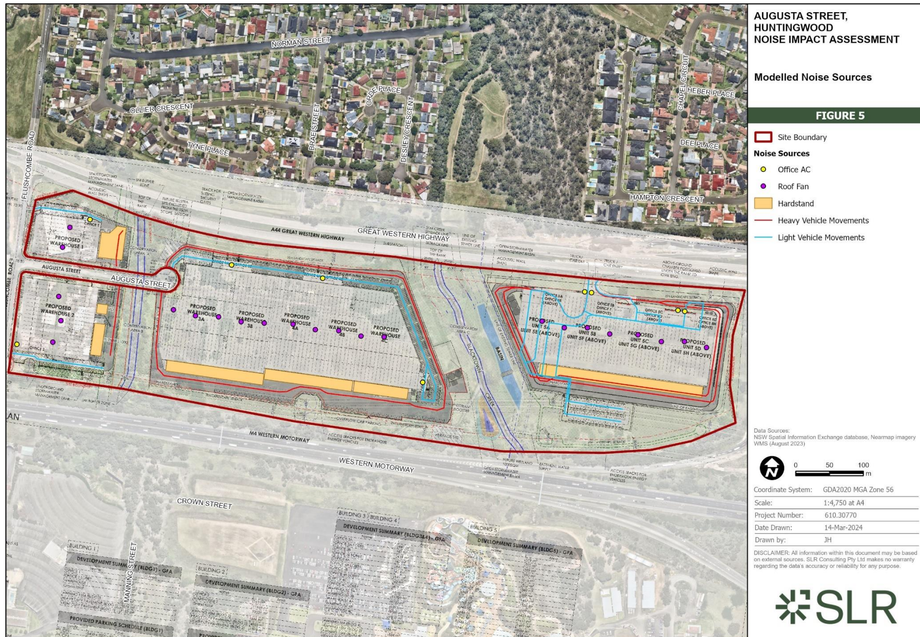
Figure 5 Modelled Noise Sources – Ground Floor and Overview
