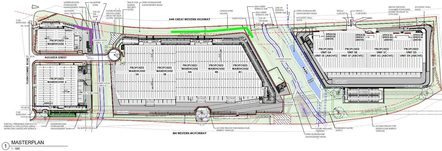
Figure 12 3 m Wall and Noise Berm Locations
